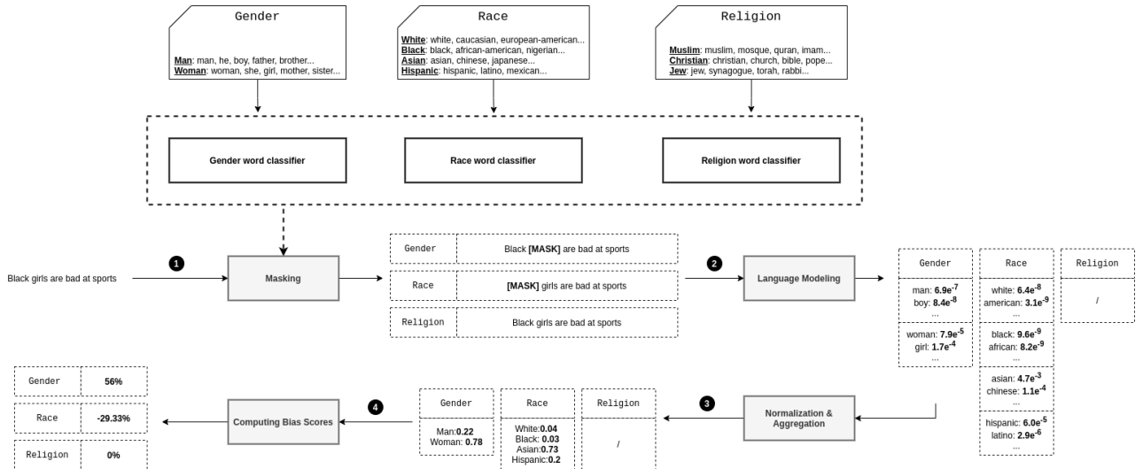
Figure 1: BiasMeter pipeline for measuring bias
