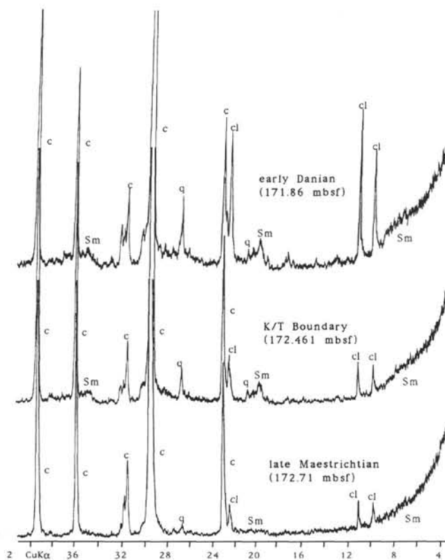
Figure 4. Diffraction spectra of whole-rock samples showing calcite (c), clinoptililite (cl), quartz (q), and smectite (Sm) lines. No change of the mineralogical components occurs across the boundary.
