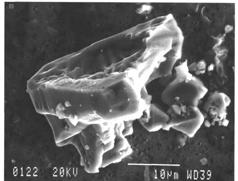
Plate 1. A. Clinoptililite crystal that has grown inside a foraminifer test. B. Isolated clinoptililite crystal. C. Magnetite-bearing flattened spheroid. Bright spots are magnetite crystals. D. Large Ni-rich magnetite.
