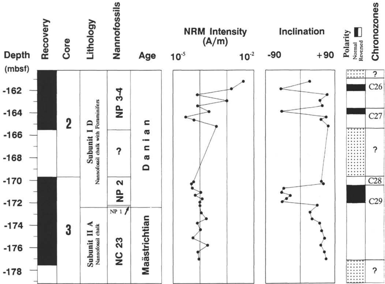
Figure 7. Maestrichtian/Danian boundary magnetostratigraphy of Hole 761C.
