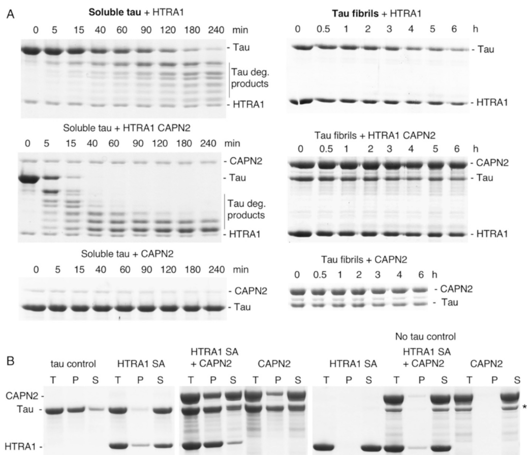
Fig. 3. Proteolysis of tau protein. (A) Left , proteolysis of soluble tau. 5 \mu M tau was incubated with 0.5 \mu M HTRA1 or 0.5 \mu M CAPN2 or with HTRA1 CAPN2 at 37°C in 50 mM Tris HCl, pH 8. Samples were taken at the time points indicated and analyzed by SDS-PAGE. Right , proteolysis of tau fibrils. Digests were performed as described for soluble tau except that 2.5 \mu M final concentration of tau fibrils and HTRA1/HTRA1-CAPN2 were used. (B) Sedimentation assay of tau fibrils. Tau fibrils were incubated with equimolar amounts of proteolytically inactive HTRA1 S328A (HTRA1SA) or CAPN2 or HTRA1 CAPN2 followed by ultracentrifugation. Subsequently, samples before centrifugation (T, total) of pellet (P) and supernatant (S) fractions were subjected to SDS-PAGE and Coomassie staining. *CAPN2 fragment. Note that CAPN2 does not digest tau because the buffers used did not contain \text{Ca}^{2+} .
