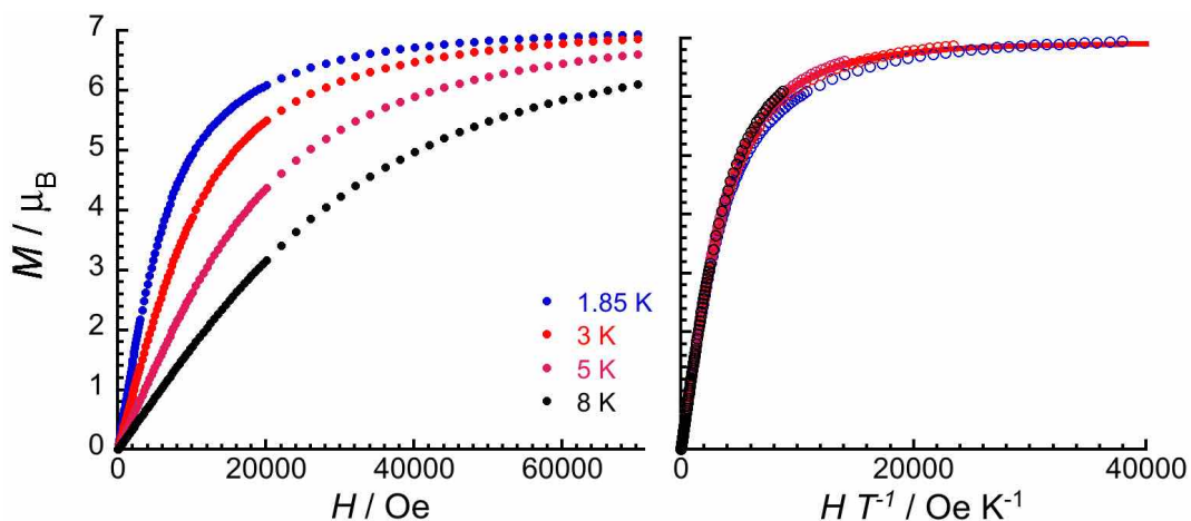
Fig. S17 Field dependence of the magnetisation for 1-Gd at low temperatures between 1.85 and 8 K with applied magnetic field from 0 to 7 T. The magnetization data are shown as a M versus H plot on the left and as a M versus H/T plot on the right (field sweeping rates: 80 Oe/min between 0 and 0.1 T, 170 Oe/min between 0.1 and 0.3 T, 400 Oe/min between 0.3 and 1 T, 830 Oe/min between 1 and 2 T, 2800 Oe/min between 2 and 7 T). At 1.85 K and 7 T, the magnetization reaches a value of 6.94 \mu_B . The solid red line is the best fit of the experimental M versus H/T data to the S = 7/2 Brillouin function with g = 1.98(3) .
