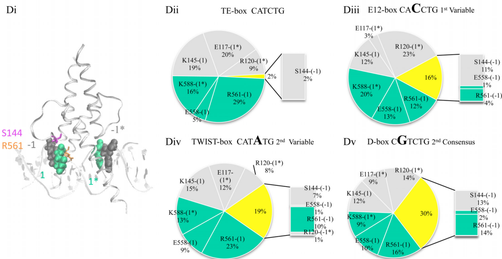
Figure 6. Binding of the TE complex to various active and modified E-box sequences, namely the E12-, TWIST- and D-boxes. (A) Plots represent the distances (Å) between the asparagine and lysine N125-K145 residues of TWIST1 and the N566-K588 residues of E12 as a function of time (total time = 10 ns, 1 frame per 10 ps) for the four (i) TE, (ii) E12, (iii) TWIST and (iv) D models during the MD simulations. These distances were estimated during the MD simulations using the VMD 1.9.1 software (Graph of Labels Bonds). The lengths of H-bond interactions were represented via GraphPad Prism 5: 'smooth, differentiate or integrate curve, with 8 neighbours'. (B and C) All cumulated occupancy values of the H-bonds were calculated as described in the Materials and Methods section. Briefly, H-bond interactions are assigned a value according to the distance between their atomic donors/acceptors during the time (the 10 ns of the MD)(interactions score 1 if their distance is under 2.10 Å, and 0 if above). Higher occupancy values being obtained for shorter and, therefore, more stable interactions. (SI function: SI(test_logic; value_if_true;value_if_false) with logic test: '<2.10', value of 1 if true and 0 if false; NB.SI function: NB.SI(range; criterion)). The calculations were carried out using Excel. (B) (i) 3D representation of the TE dimer highlighting the position of the interaction between the asparagine and lysine residues N125-K145. (ii) The horizontal bar chart represents the rate of cumulated occupancy of the N125-K145 of TWIST1 and the N566-K588 of E12, in grey and green, respectively, for the four E-box sequences. (C) Top, representation of the E-box sequence, with the forward half-site and the reverse complementary half-site in orange and pink, respectively. Table showing the rate of cumulated occupancy of H-bonds established between the TE complex and either adjacent bases, or consensus and variable bases of TE-, E12-, TWIST-, and D-box sequences. The percentage of variation compared to the TE-box is reported in brackets. (D) (i) 3D in silico representation of the TE complex bound to DNA. The proximal flanking ((-1) and (-1*)) and first ((+1) and (+1*)) bases of the E-box are represented in green and grey VDW, respectively. The serine S144 and arginine R561 residues are highlighted in magenta and orange, respectively. (ii-v) The pie charts show the percentages of cumulated occupancy of H-bonds established between residues of TWIST1 (grey) and E12 (green) and DNA bases during the (ii) TE-, (iii) E12-, (iv) TWIST- and (v) D-box MD simulations. Occupancies of H-bonds established with the proximal flanking ((-1) and (-1*)) bases are represented in yellow, while the bar charts highlight the exact residues binding to those bases. The H-bonds established with the first consensus ((+1) and (+1*)) bases of the E-box are represented in grey and green for the TWIST1 and the E12 residues, respectively.
