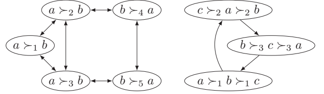
Figure 2: Left: A strongly connected influence network and a stable profile. PPD does not converge to consensus despite the fact that the majority relation is (trivially) acyclic. Right: A simple cycle influence network and a preference profile with a cyclic majority relation. PPD converges to consensus (see Section 5.2).
