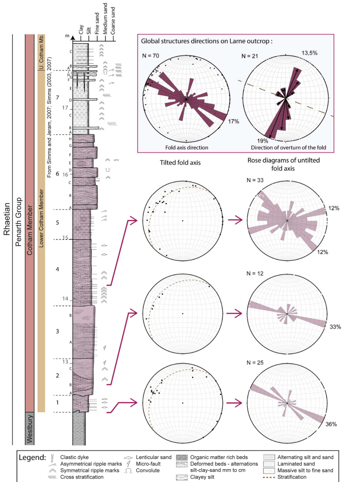
Figure 2. Detailed log section of the Waterloo Bay foreshore, Larne. SSDs are observed in units 1 to 6 (beds in purple). Plots on the left correspond to fold axes with the present day dip. Rose diagrams on
