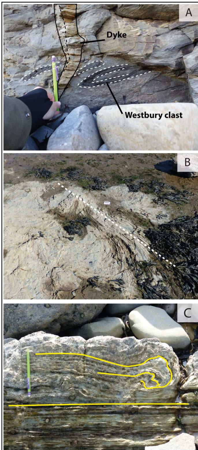
Figure 6. SSDs in SW Great Britain (Bristol Channel Basin). (A) Deformed clast of the Westbury Formation within the base of the lower Cotham Member at Lavernock Point (unit 2A). The clastic dyke postdates the recumbent fold formation. (B) Isoclinal fold axis in the lower Cotham Member on the foreshore (unit 2E), Lilstock. (C) Recumbent fold in the lower Cotham Member (unit 2D) at St Audrie's Bay.
