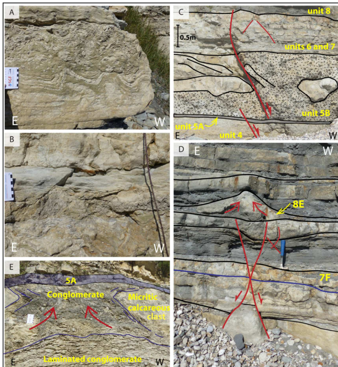
Figure 8. SSDs observed in South Devon (A) Fluid escapes features highlighted by convolute bedding at the top of a debris flow, unit 3A, Pinhay Bay. (B) Synsedimentary fault between units 3C and 3D at Pinhay Bay. Unit 3C is injected along the fault and forms a dome structure. (C) Normal fault affecting units 5B to 8E at Pinhay Bay. The fault limits the liquefaction of the slumped unit 5B (shown by stippled pattern). (D) Normal fault with injection feature at the top of unit 8E. (E) Massive injection features within a matrix-supported conglomerate throughout unit 4C at Charton Bay. Unit 5A is not affected (marked by coloured overlay).
