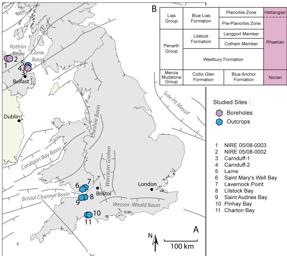
Figure 1. Tectonic framework of the UK at the Triassic–Jurassic transition. A: Location of studied sites. The faults which mark the different Permo-Triassic basins are those defined by Holdsworth et al. (2012). B: Lithostratigraphy of the Triassic-Jurassic boundary deposits in the UK. After Warrington et al. (1994) and Mitchell (2004).
