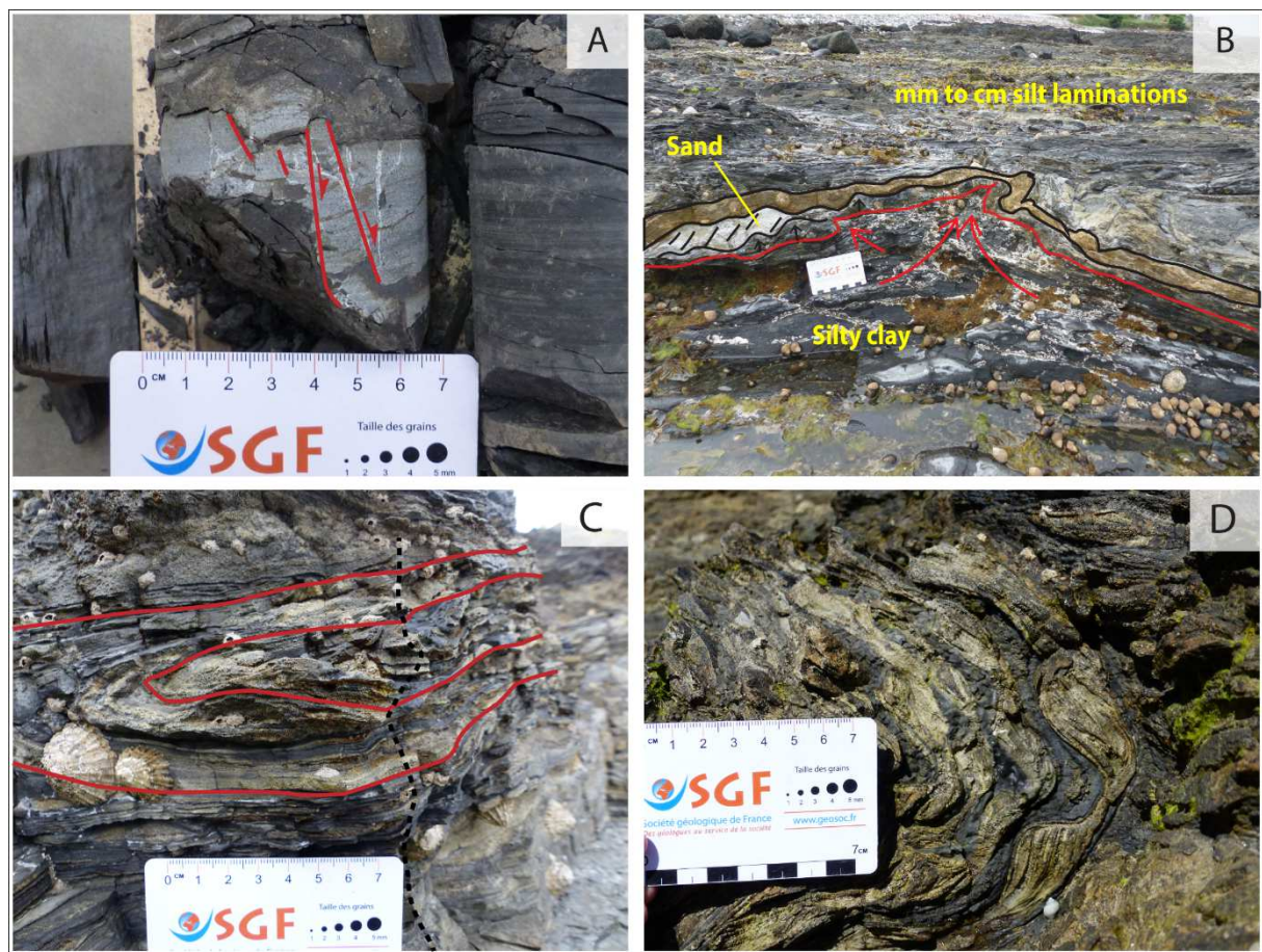
Figure 3. SSDs observed in Northern Ireland. (A) Synsedimentary micro-faults in the Westbury Formation, NIRE 05/08-0003 core. (B) Diapir injection structure at the boundary between the Westbury Formation and the Cotham Member, Waterloo Bay. (C) Recumbent fold in the lower Cotham Member, Waterloo Bay. (D) Second generation of folds and boudinage in a larger fold, Waterloo Bay.
