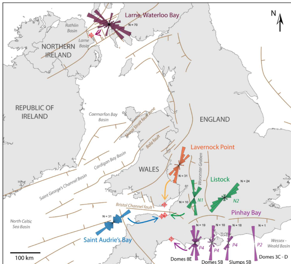
Figure 9. Main orientations of deformation structures observed in each outcrop in the UK. N: number of data. N1 and N2 in Listock, P2 and P4 in Pinhay Bay refer to the two deformed levels recognised in these sites.
