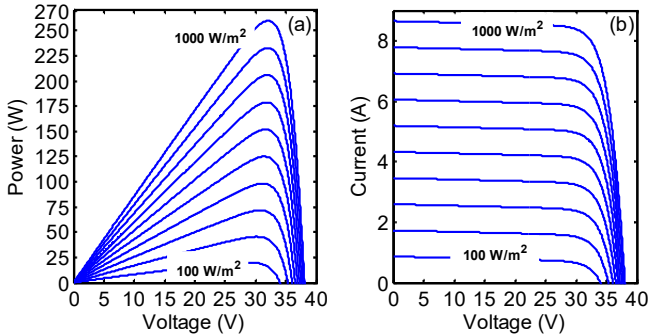
Fig. 2 – Characteristics of the used IFRI260-60 PV panel at 25°C for different irradiance levels (graphs plotted with step of 100 W/m²): (a) power-voltage (P-V) curves; and (b) current-voltage (I-V) curves.
