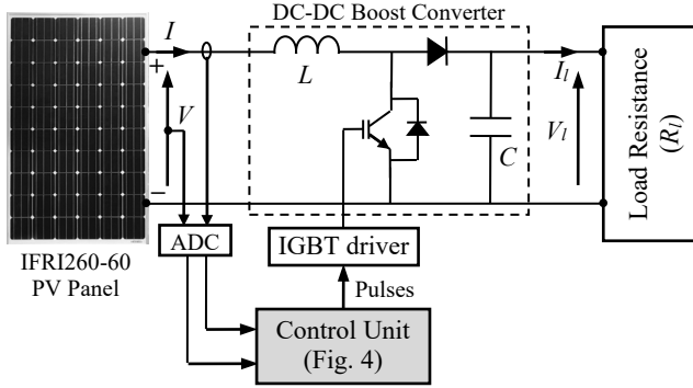
Fig. 1 – Simplified block diagram of the controlled PV system.
