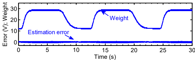
Fig. 12 – Evolution of the weight and estimation error in the ANC method under low to medium irradiance with fast profile.
