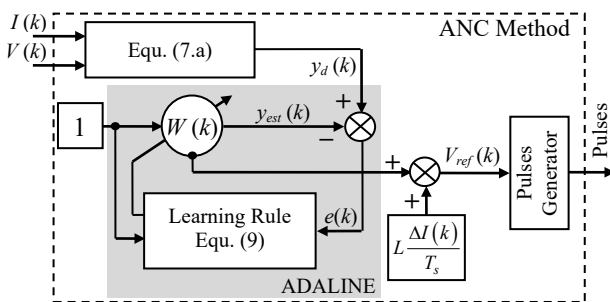
Fig. 4 – Block diagram of the proposed ANC method.
