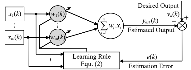
Fig. 3 – ADALINE topology.
