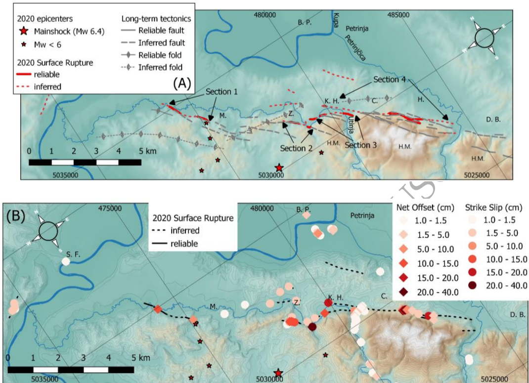
Figure 7: Maps representing the surface rupture, (A) with the sections showing reliable and inferred traces, stars represent the mainshock and main events of the sequence (section 1: Međurače; section 2: Župić; section 3: Križ; section 4: Cepeliš) and (B) with the offsets measured in the field (B). Notice that the separation between the sections 1 and 2 is due to a lack of observation (mine fields). The database is available in Supplementary Material (S2.1). S. F.: Stari Farkašić, M.: Međurače, Z.: Župić, B. P.: Brest Pokupski, K. H.: Križ Hrastovački, C.: Cepeliš, H.: Hrastovica, H. M.: Hrastovica Mountains, D. B.: Donja Budičina.
