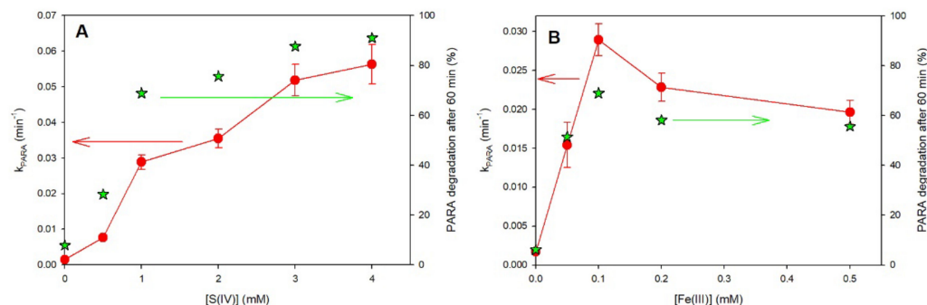
Figure 4. First order rate constant of PARA degradation ( k_{\text{PARA}} ) (filled circles) and degradation efficiency in percentage after 60 min (green stars) as a function of S(IV) (A) and Fe(III) (B) concentrations under UVA in aerated solutions. Conditions: [\text{PARA}]_0 = 10 \mu\text{M} , [\text{Fe(III)}]_0 = 0.1 \text{ mM} , [\text{S(IV)}]_0 = 1.0 \text{ mM} , \text{pH}_{\text{init}} = 7.0 .
