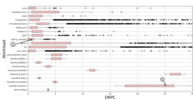
(a) DRPC distributions per workload
