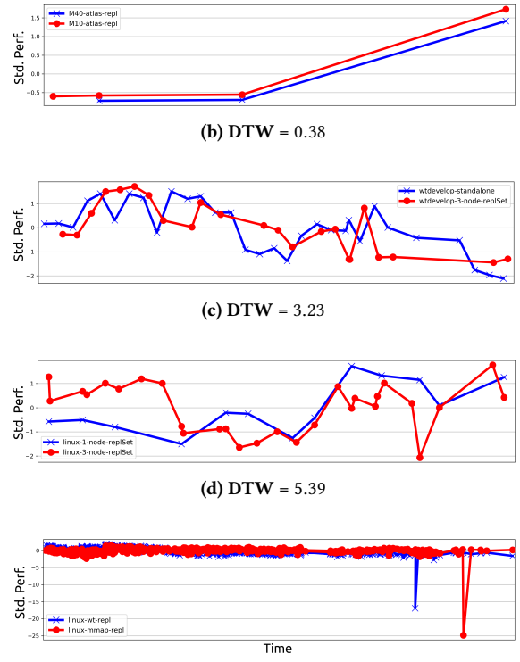
(e) DTW = 15.31
