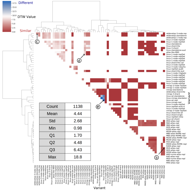
(a) Heatmap of average DTW between times series related to different variants of hardware
