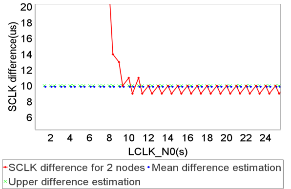
Figure 8: Mean and upper bound estimation of the shared clock difference for the 2-node topology for a 20ppm drift.
