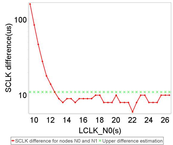
Figure 9: Measured difference of the shared clocks (in log scale) for a 2-node topology.
