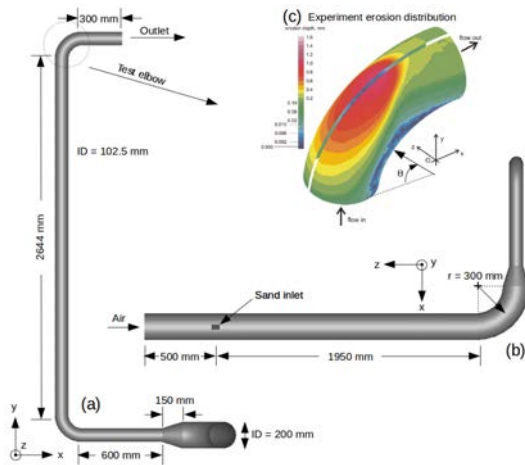
Figure 1: (a) and (b) Experiment set-up of Solnordal et al. (2015); (c) Contour of erosion depth after passage of 200 kg sand.
