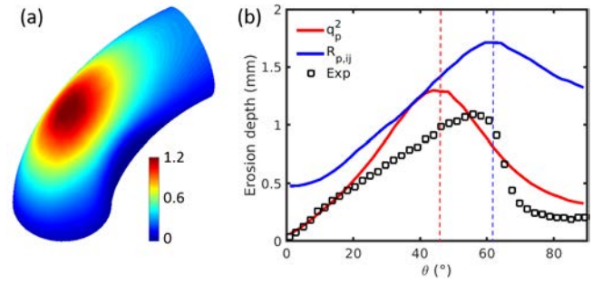
Figure 2: (a) Contour of erosion depth with the particle turbulence model q_p^2 ; (b) Erosion depth profiles on the elbow extrados for two different particle turbulence models, the dashed lines correspond to the erosion peak location.
