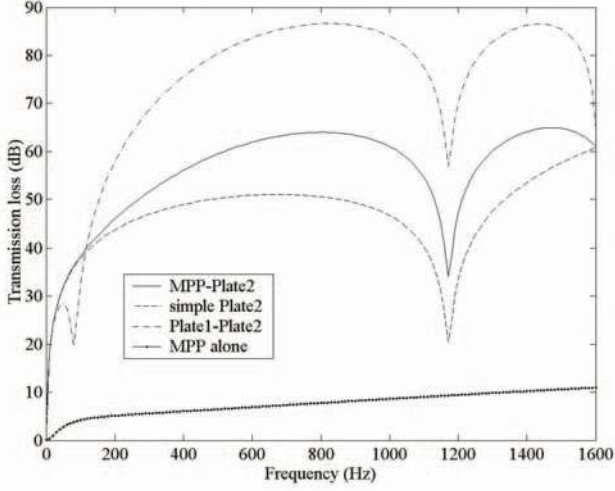
Figure 12. Transmission loss at 45^\circ oblique incidence – MPP + thick solid plate of 20 mm thickness. The curves represent the basic system (MPP + solid plate), simple plate alone, two simple plates and MPP alone. The MPP is made of steel, hole diameter 0.5 mm, thickness 1 mm, perforation ratio 0.55%. The steel solid plate is 0.7 mm thick. The air gap is 0.15 m.
