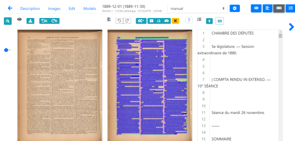
Figure 3: eScriptorium interface
