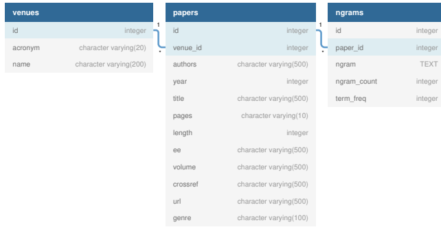
Figure 2: Relational database schema of the dataset.
