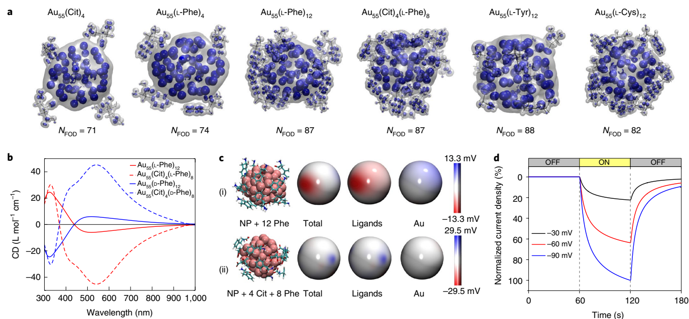
Fig. 4 | Photocurrent generation via plasmon-driven ejection of electrons to the particle-medium interface. a , FOD for different NP-ligand models. All FOD isosurfaces were obtained using 0.002 e/\text{Bohr}^3 and 0.02 e/\text{Bohr}^3 isovalues for semitransparent grey isosurfaces and opaque blue isosurfaces, respectively. Grey denotes the regions that can be accessible to ejected electrons; blue denotes the regions where they are more likely to be localized. b , CD spectra calculated for NPs decorated with either Phe or a mixture of Cit and Phe. c , DFT simulation of the average transient electrostatic potential distribution of \text{Au}_{55}(\text{L-Phe})_{12} and \text{Au}_{55}(\text{Cit})_4(\text{L-Phe})_8 under excitation by 808 nm photons. These results directly confirm that both systems produce a non-uniform electrostatic potential of tens of millivolts in the nearby solution, and the adsorbed ions are expected to move in response to the corresponding electric field. \text{Au}_{55}(\text{Cit})_4(\text{L-Phe})_8 shows a higher photoexcitation potential under light because it has a stronger solvated-electron-holding capacity. The spherical surfaces around the NPs correspond to the regions in which ions are expected to be adsorbed onto their surfaces. The total electrostatic potential was split into the contribution from the NPs and the ligands. d , The normalized photocurrent difference generated by the different transmembrane potentials driving the directional ion transport calculated with finite element simulations; the photocurrent kinetics were nearly identical to those observed experimentally.
