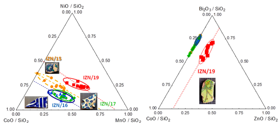
Figure 8. Ternary scatter plots of CoO, NiO, and MnO (left) and CoO, \text{Bi}_2\text{O}_3 , ZnO (right) normalized by \text{SiO}_2 found in the blue coloured areas (#X: spot number, see Appendix A). Lines and ellipses are drawn as a guide for viewing.
