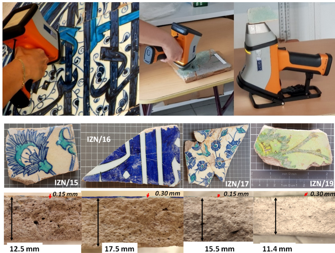
Figure 1. Examples of on-site use of hh-XRF instrument: ( top-left ) on-site measurement of the tile panel of Üç Şerefeli Mosque in Edirne, and ( centre ) and ( top-right ) measurements at the Iznik Tile Kilns Excavation' house; ( bottom ), representative images of the sherds of tiles. IZN/15, IZN/16, and IZN/17 belong to the group of “blue-and-white” tiles, while IZN/19 is known as a Rhodes work. Cross-sections (from Bilge Çubukçu) show the thicknesses of the glaze and paste.
