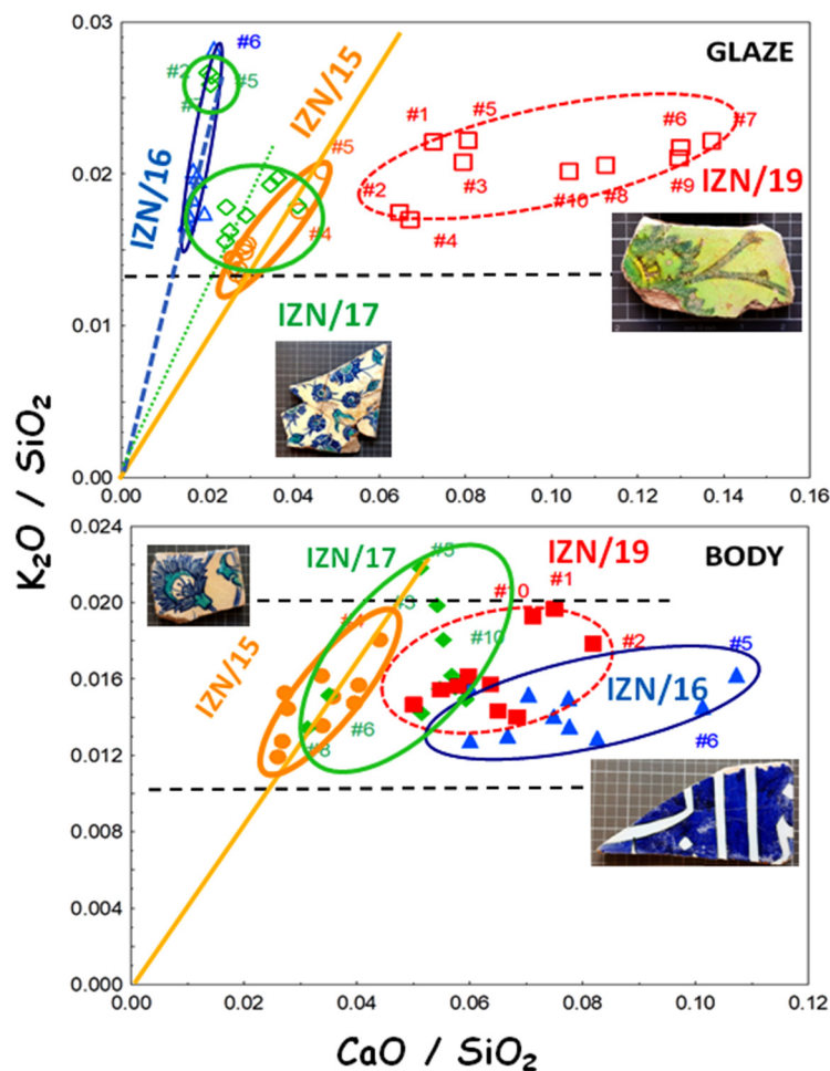
Figure 6. Binary scatter plots of K_2O/SiO_2 versus CaO/SiO_2 in the glaze (upper) and body (bottom). Lines are drawn as a guide for viewing (See Figure 4 for labels, #X: spot number, see Appendix A).
