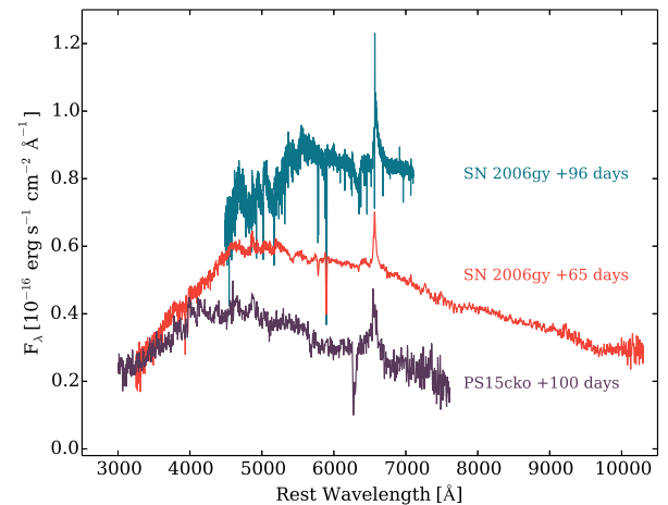
Figure 4. Top: the light curve of the luminous PS15cko compared to two three other superluminous Type II SNe. No host reddening has been applied to PS15cko. Bottom: spectral comparison of PS15cko with the two spectra of SN2006gy. Each spectrum has been corrected for foreground extinction only, since the host extinction to PS15cko is uncertain. The light curves and spectral comparison indicate this is a luminous Type II SN.
