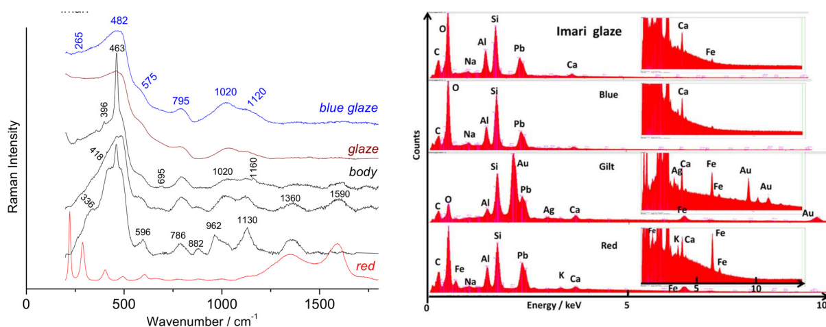
Figure 9. Representative Raman spectra (left) and EDXS spectra (right) recorded on Imari-style Chinese plate (Figure 2f): blue and colorless glaze surface, body section and red area paint.
