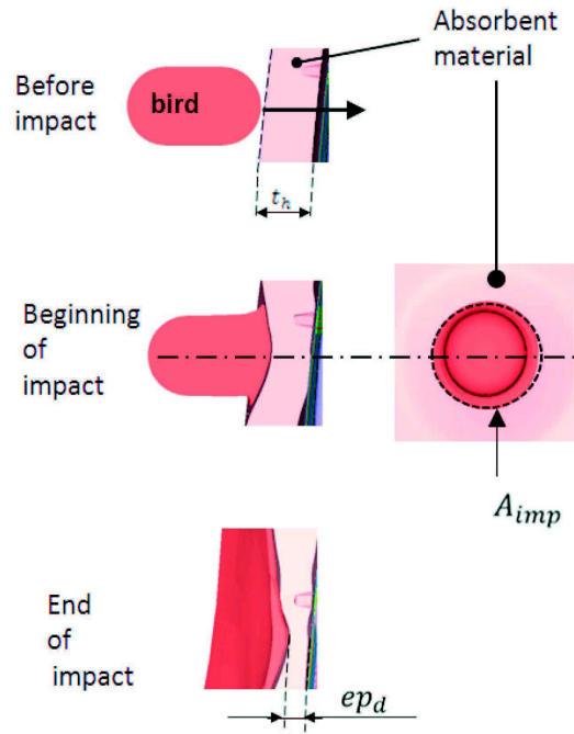
Fig. 5. Geometrical parameters.
