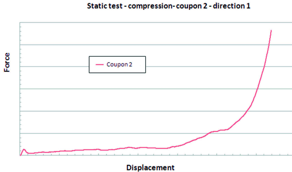
Fig. 6. Static test in compression for coupon number 2 with force versus displacement curve for material direction number 1.
