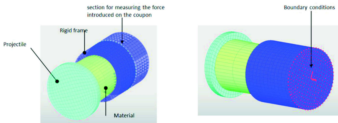
Fig. 7. Numerical finite element model (virtual testing).
