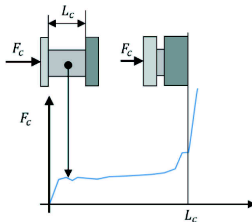
Fig. 3. Compressive curve force versus displacement of the honeycomb material.
