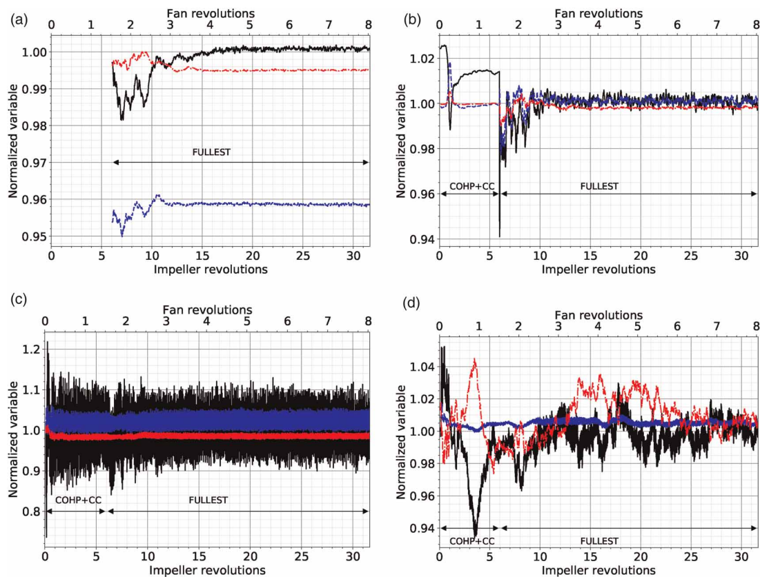
Figure 5. Convergence plots of normalised integral values for (solid black) \dot{m} , (dash-dotted red) T_t and (dashed blue) P_t at four different cross-sectional positions noted in yellow in Figure 1e. Values are normalised by the ones from the thermodynamic cycle. (a) Secondary flow outlet. (b) Impeller inlet. (c) Axial diffuser trailing edge. (d) Combustion chamber exit.
