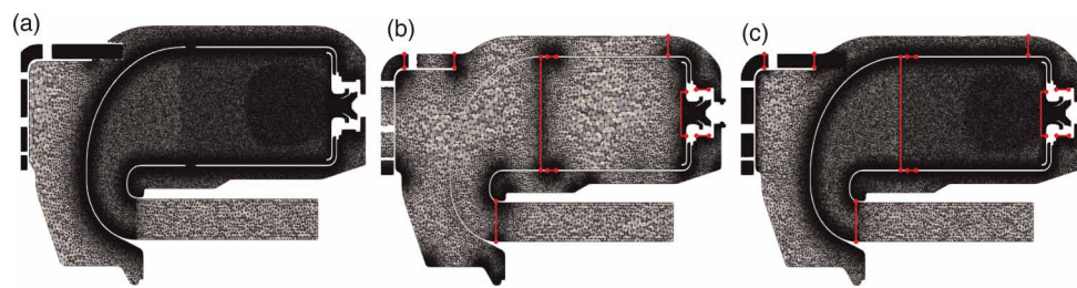
Figure 3. Meridional cut of the mesh for the diffusers and the combustion chamber. (a) Target mesh (1 sector). (b) Coarse mesh (360°). (c) Adapted mesh (360°).
