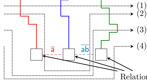
(b) Widget for the relator abc = 1_G . From top to bottom, the words associated with the paths (1) to (4) are respectively abc = 1_G , aa^{-1}(ab)c = 1_G , (ab)c = 1_G and 1_G . For clarity, the relation tiles are not adjacent on the figure
