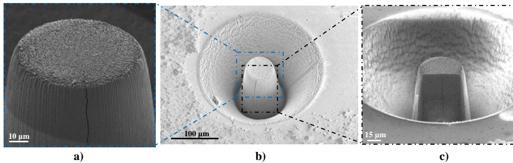
Fig 4. Ex-situ characterization after mechanical loading of the 8YSZ pillar sintered at 1270^\circ\text{C} (low porosity): a) SEM image of a longitudinal crack on the edge of the pillar, b) SEM image of the tested pillar, c) FIB-SEM cross section showing the large crack in the bulk of the pillar.
