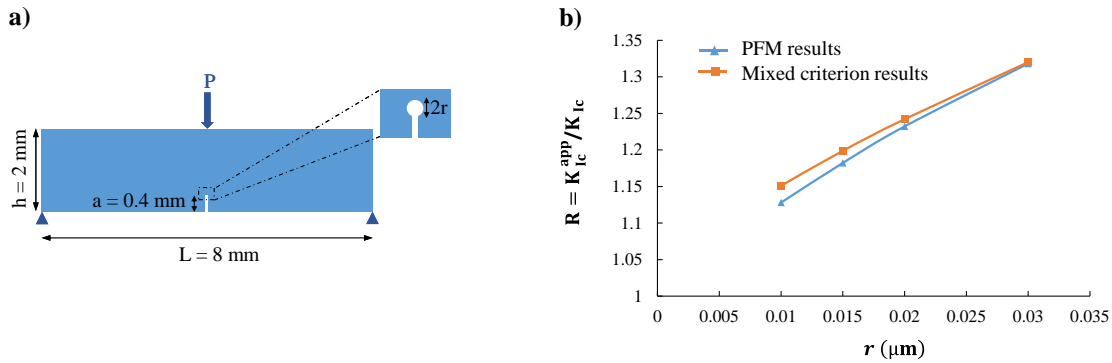
Fig 8. Three point bending test on a sample with a crack blunted by a cavity: a) implemented geometry, b) comparison between PFM and mixed criterion results for 8YSZ material.
