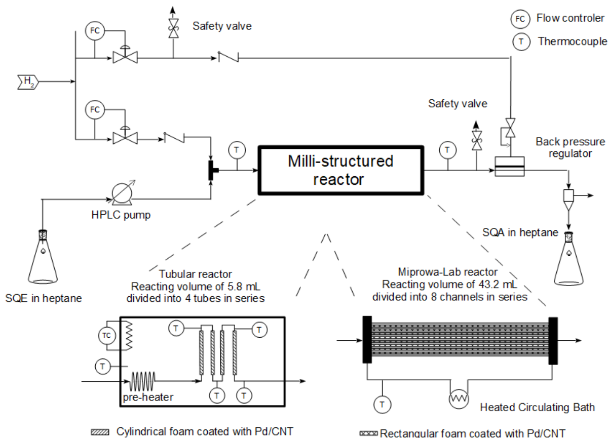
Scheme 1. Experimental setup for the reduction of SQE in flow using milli-reactor
