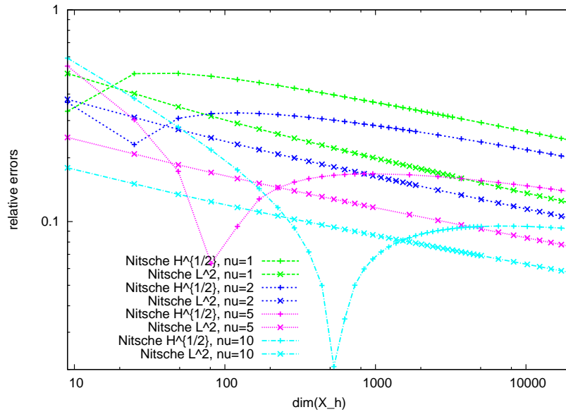
Figure 5.2: Skew-symmetric Nitsche method ( \sigma = -1 ): relative error curves (upper bounds (5.2) and (5.3)).
