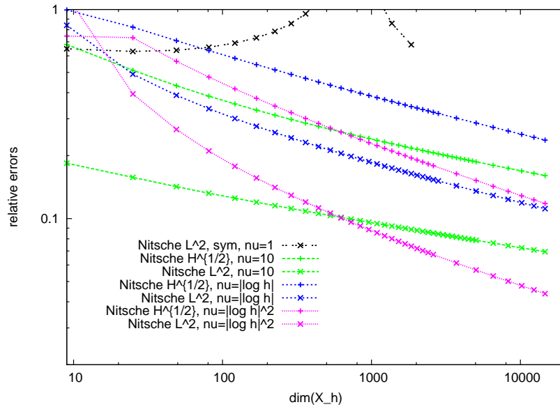
Figure 5.4: Symmetric Nitsche method ( \sigma = -1 ): relative error curves (upper bounds (5.2), except for \nu = 1 , and (5.3)).
