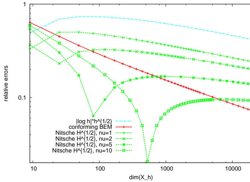
Figure 5.1: Skew-symmetric Nitsche method ( \sigma = -1 ): relative error curves (upper bound (5.2)). Comparison with conforming BEM.
