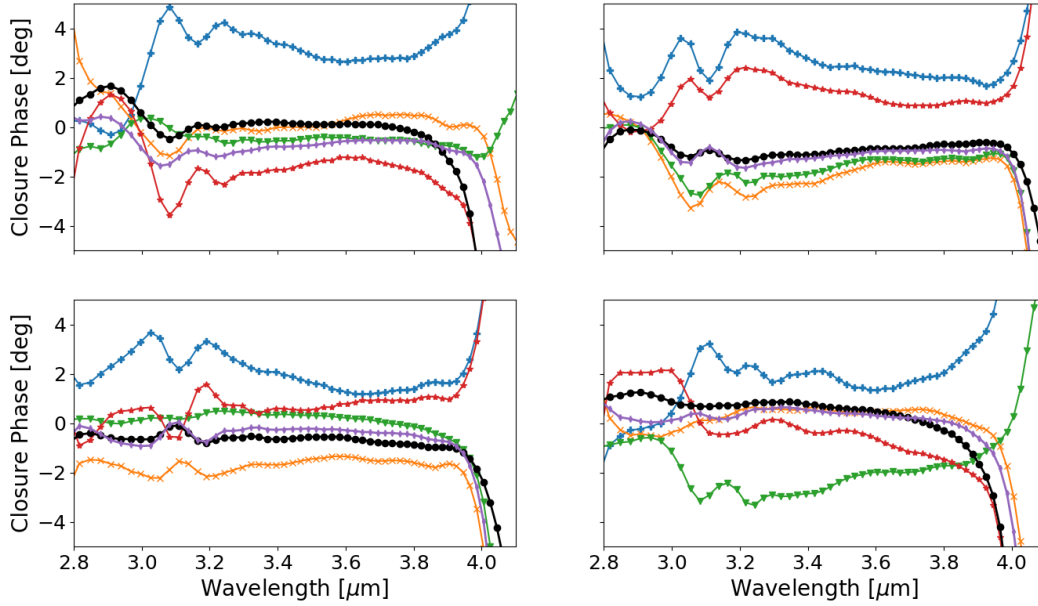
Fig. 14. Four closure phases obtained on a bright star, IRAS 10153-5540, as a function of the wavelength. The blue(+), red(*), green(∇), and orange(x) lines represent the CP for the different BCD position calibrated by VV396 Cen. The black(●) line represents the CP corrected by the BCDs only. The purple(◊) line represents the CP of IRAS 10153-5540 calibrated by VV396 Cen and corrected by the BCDs.
