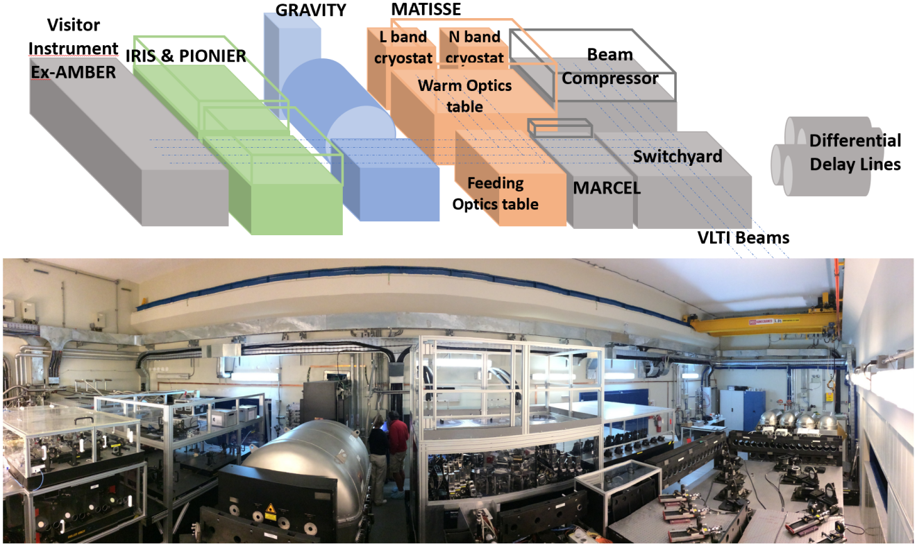
Fig. 1. MATISSE in the VLTI focal laboratory. Top : layout of the instruments and devices. In front of MATISSE, the feeding optics table reflects either four UT or AT beams towards the instrument, after their transportation through the VLTI optical train. Bottom : view of MATISSE warm optics table called the WOP (and its cover) in the foreground.
