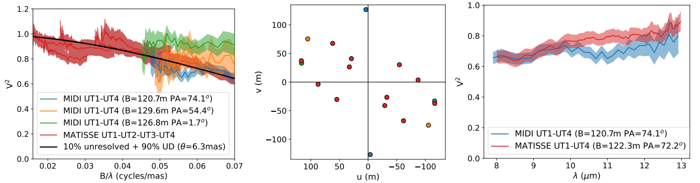
Fig. 22. Comparison between MATISSE N band and MIDI data obtained on the classical Be star \alpha Arae using the UTs. Left: all data plotted as a function of the spatial frequency with a best unresolved + uniform disk model. Centre: corresponding uv plane coverage with the same colours for MIDI and MATISSE observations. Right: data plotted as a function of the wavelength for two similar baselines in terms of length and orientation.
