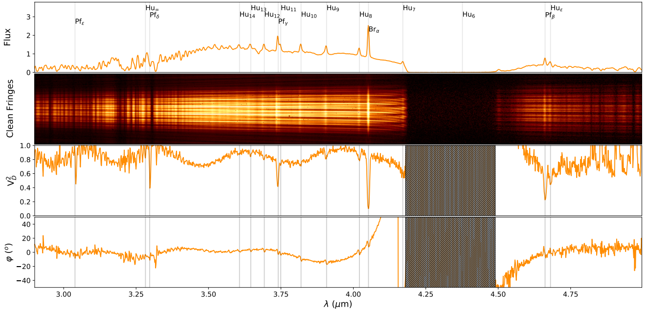
Fig. 29. L&M bands medium resolution ( R \sim 500 ) observation of the Be binary \delta Cen obtained in GRA4MAT mode. From top to bottom: source spectrum, cleaned 10 s frame (i.e. with the mean sky removed) in the interferometric channel, differential squared visibility for one of the six baselines, and corresponding differential phase. The gap between the L and M band is shown in grey in the visibility and phase plots. The source spectrum shows a rich collection of hydrogen emission lines in Br \alpha and the Humphrey and Pfund series. The interferometric channel of MATISSE composed of straight and stable high contrast fringes from 2.9 to 4.9 \mu m shows a collection of bright source emission lines and dark telluric absorption lines.
