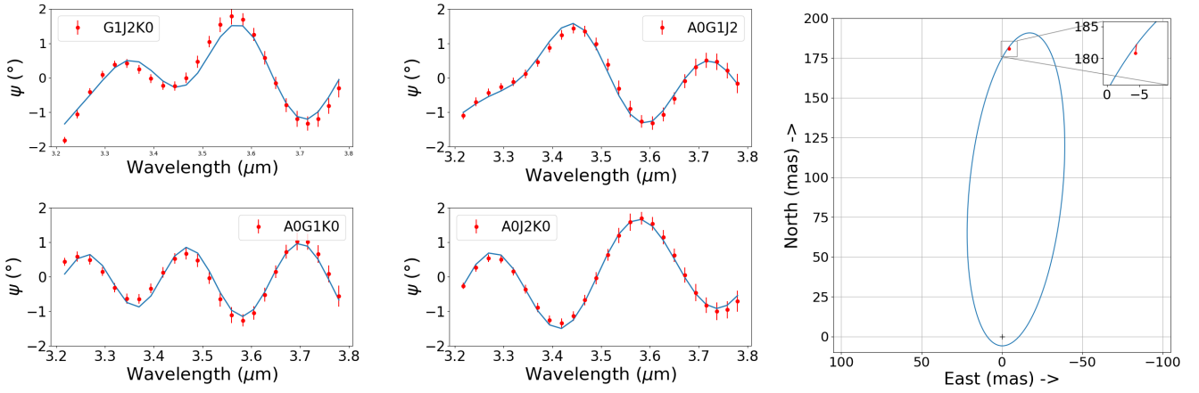
Fig. 28. Observation of \delta Sco with MATISSE in L band. Left panels: \delta Sco closure phases (red) and the best-fit binary star model (blue). Right panel: comparison between the Tycner et al. (2011) orbit (blue) and our astrometric point (red).
