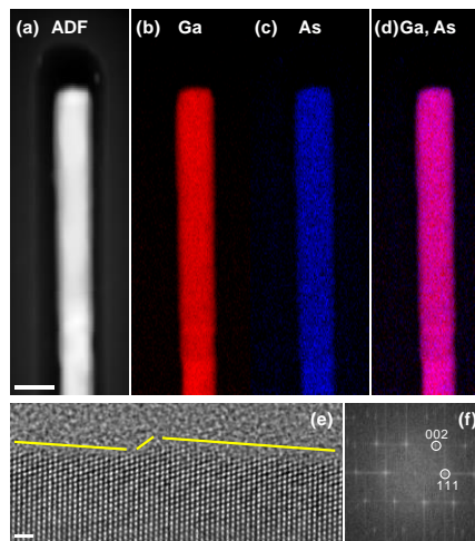
Figure 6. (a) STEM-ADF image acquired simultaneously with an EELS spectrum image leading to the elemental maps of (b) Ga, (c) As, and (d) Ga+As; scale bar: 100 nm. (e) High resolution TEM image of the NW after decapping of the As shell; scale bar: 1 nm. The yellow lines follow the facets and are guides for the eye. (f) FFT performed on the NW shown in (e).
