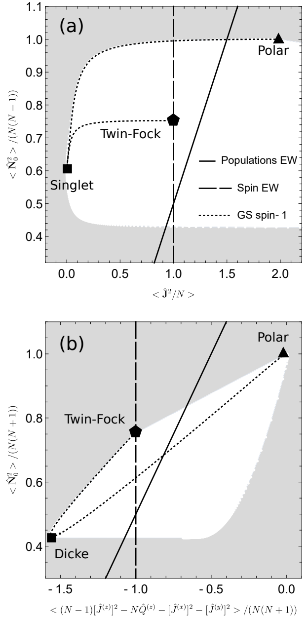
Figure 1: (a) Comparison of the population-based witness [Eq. (6)] (solid line) with the SSI \text{Var}(\hat{\mathbf{J}}) \geq Nj (dashed line) for spin-1 states ( N = 100 atoms). The light grey area are data points which cannot be achieved (see text and Appendix D). The dotted line indicates the ground state of Eq. (5) for both antiferromagnetic interactions ( c = 1 ), varying the quadratic Zeeman term ( -10 \leq q \leq 10 ). Three representative states are also indicated: the polar state |0, N, 0\rangle ( q \rightarrow \infty ) which is separable, the spin singlet s.t. \hat{\mathbf{J}}^2|\Psi\rangle = 0 ( q = 0 ), and the twin-Fock state |N/2, 0, N/2\rangle ( q \rightarrow -\infty ). (b) Comparison of the population-based witness [Eq. (7)] with a related SSI (see text) for spin-1 states. Graphical conventions as in panel (a). Here, the ground state is computed for ferromagnetic interactions ( c = -1 ). At q = 0 , we obtain the Dicke state \hat{\mathbf{J}}^2|\text{Dicke}\rangle = N(N+1)|\text{Dicke}\rangle , \hat{J}^{(z)}|\Psi\rangle = 0 .
