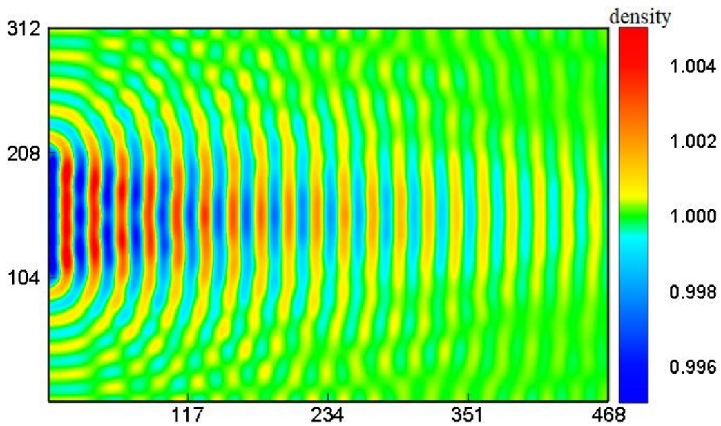
Figure 5. Density field showing sound waves propagation in the rectangular cavity after 1400 iterations for a LBM viscosity \nu = 1.21 \times 10^{-6} .
