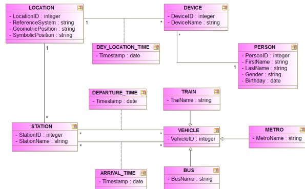
Figure 4: Mobility information.
