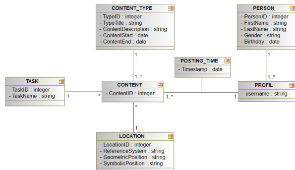
Figure 5: Crowdsourcing information.
