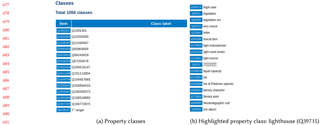
Fig. 14. Property classes: curation of properties for a particular class
