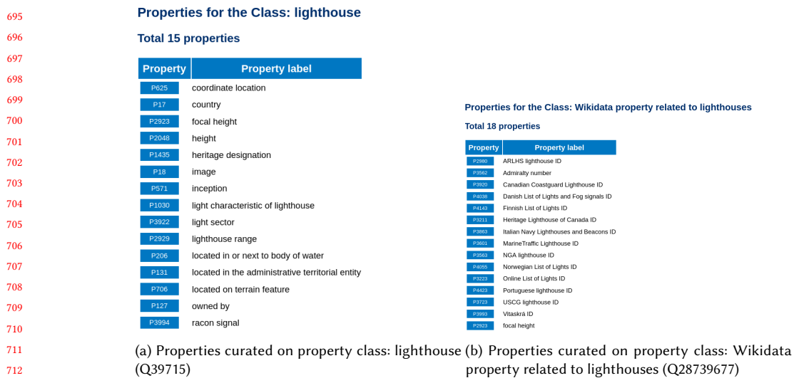
Fig. 15. Properties curated on two property classes
