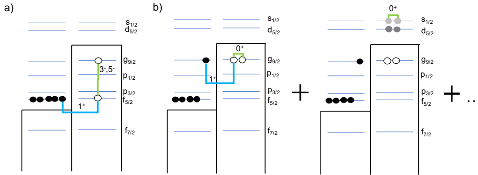
Fig. 13. Schematic representation of the doorway configurations involved in the 9/2^+ \rightarrow 7/2^+, 9/2^+, 11/2^+, ^{81g^s}\text{Ge} \rightarrow ^{81}\text{As} Gamow-Teller decay.
