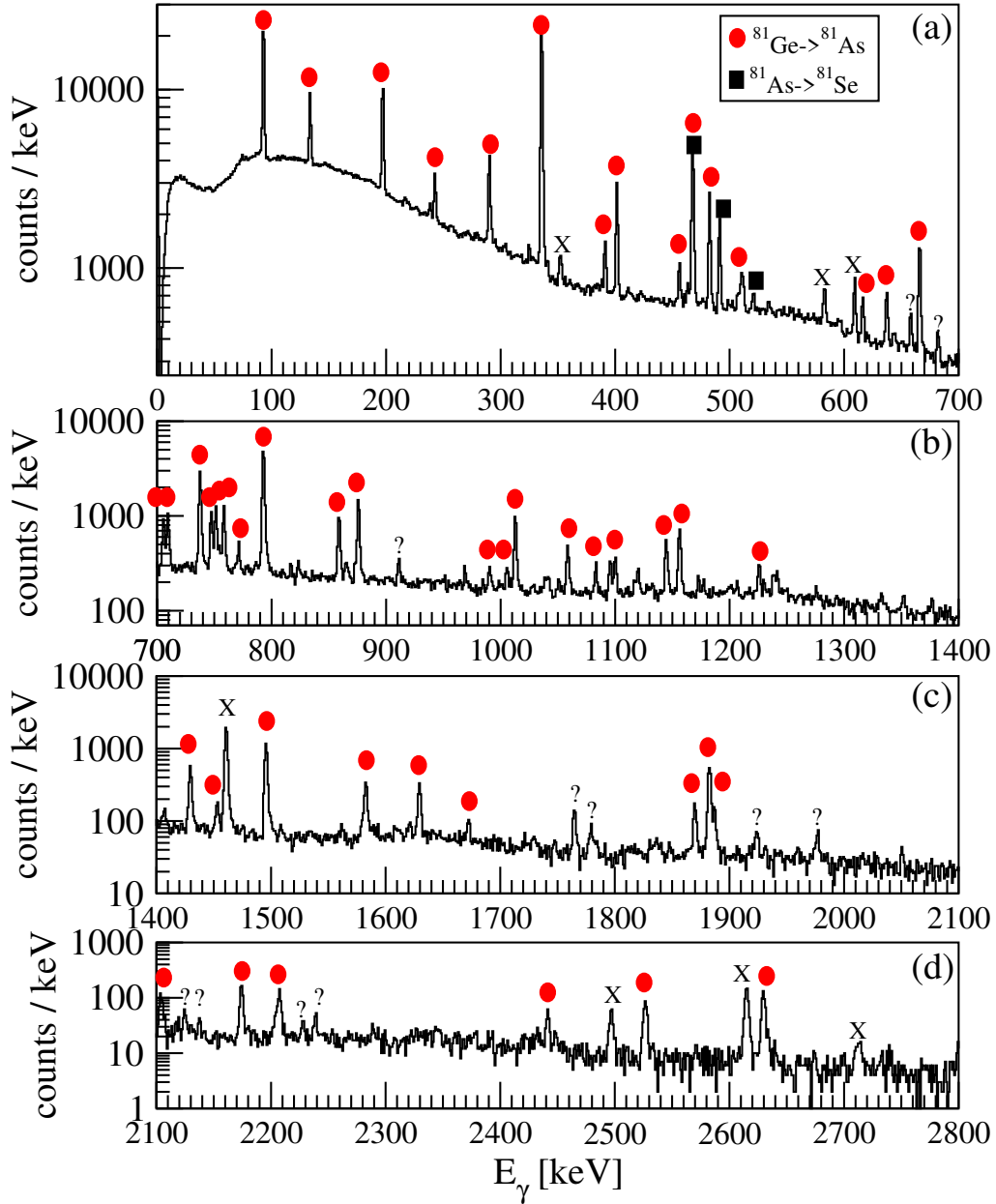
Fig. 4. Trap assisted experimental \beta -gated \gamma -ray spectrum at \nu_c = 1327846.166 Hz. (a), (b), (c) and (d) represent subsequent energy ranges 0–700, 700–1400, 1400–2100, and 2100–2800 keV, respectively. Red circles indicate transitions attributed to ^{81}\text{As} and black squares, transitions in ^{81}\text{Se} . Peaks indicated with X are considered as pollutant as their time distribution is not correlated to the beam. Finally, ? shows unidentified peaks (no coincidence, unclear time distribution).
