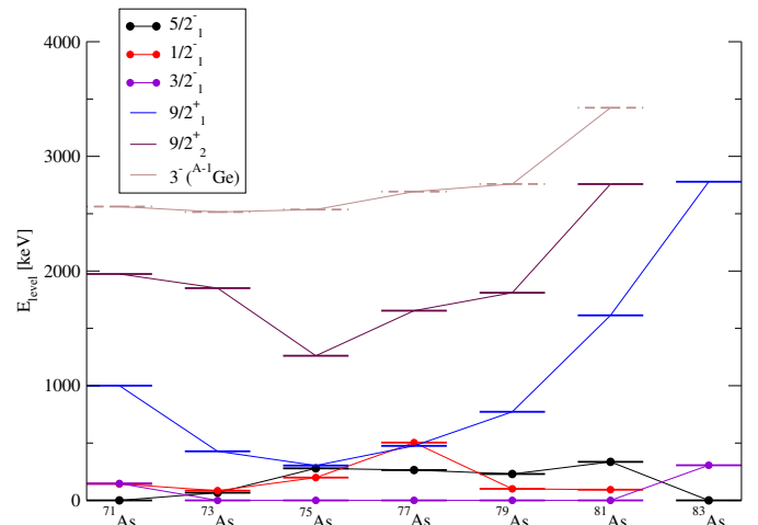
Fig. 8. Level systematics of odd-mass As isotopes. Data are taken from [35]. Circles indicate levels with a strong single-particle component seen in one-proton pick-up [37] and/or stripping [38,39] reactions.
