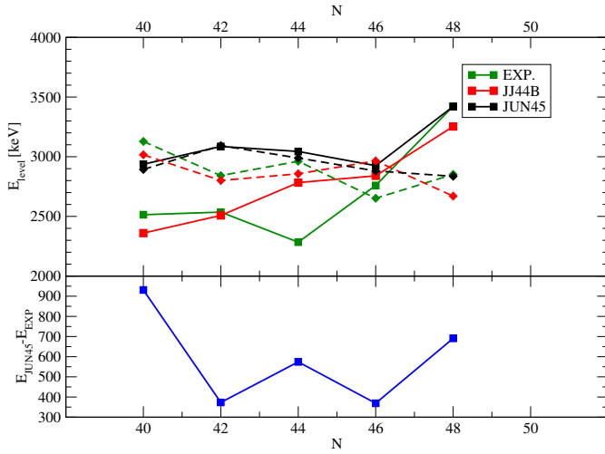
Fig. 11. Upper panel : comparison between experimental (green) and calculated 3_1^- (square, full lines) and 5_1^- (diamond, dashed lines) states obtained with two different shell-model interactions JJ44B (red) and JUN45 (black). Lower panel : difference between the experimental and (JUN45) shell model excitation energies of the 9/2_1^+ states for As isotopes.
