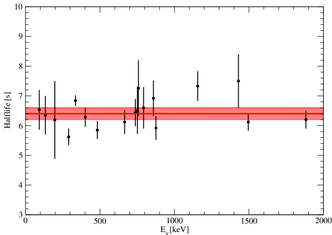
Fig. 3. The determined half-lives for the studied \gamma -ray transitions as a function of the \gamma -ray energy E_\gamma (in black). The weighted mean and its error band including both systematic and statistical uncertainties is shown in red.
