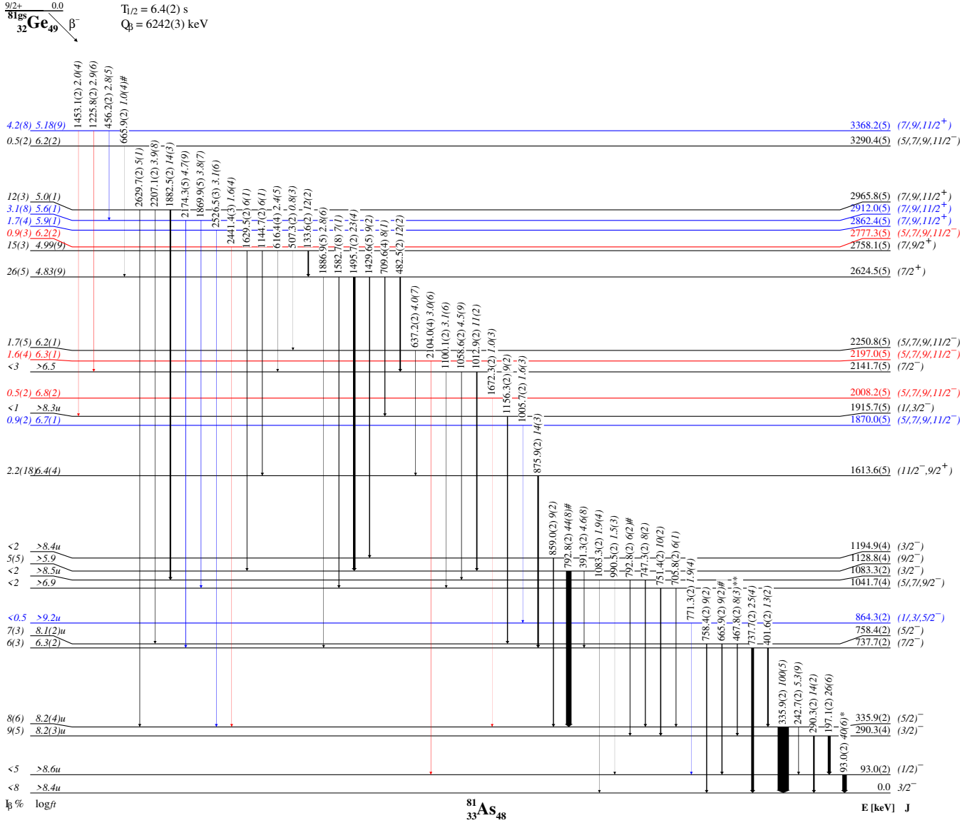
Fig. 5. ^{81}\text{Ge} \beta -decay scheme. Levels and transitions shown in black (blue) were already attributed to the ^{81}\text{Ge} ground state (isomer) decay in Ref. [14], respectively. Levels and transitions shown in red are those newly proposed from the present work. * indicates that intensity has been corrected by conversion coefficient assuming M1 multipolarity. ** indicates that intensity has been corrected taking into account the ^{81}\text{Se} transition. # are indicating intensities estimated using \gamma - \gamma coincidences for the doublets. Spin-parity notation (1/3, 5/2^-) stands for (1/2^-) , (3/2^-) or (5/2^-) .
