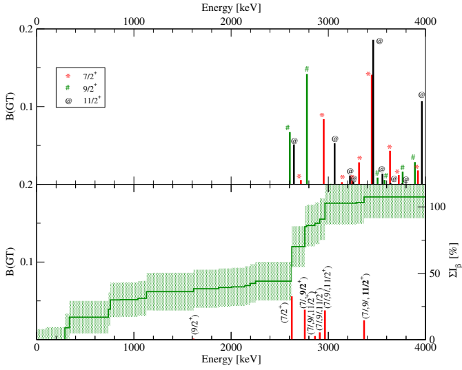
Fig. 12. Upper panel : theoretical B(GT) distribution obtained with JUN45 shell-model calculation for ^{81}\text{As} . Bottom panel : experimental results from this work for ^{81}\text{As} , the red vertical bars represent the B(GT) for allowed transitions, while the green discontinuous line represents cumulative \beta strength as a function of the energy.
