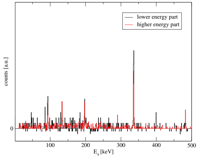
Fig. 6. Normalised \gamma spectra obtained by gating on the lower (black) or higher (red) energy part of the 793-keV peak in the \beta -gated \gamma - \gamma coincidence matrix with identical background subtraction. I(290 \text{ keV})/I(336 \text{ keV})=0.02(2) for lower energy gate and I(290 \text{ keV})/I(336 \text{ keV})=0.12(3) for higher energy part.
