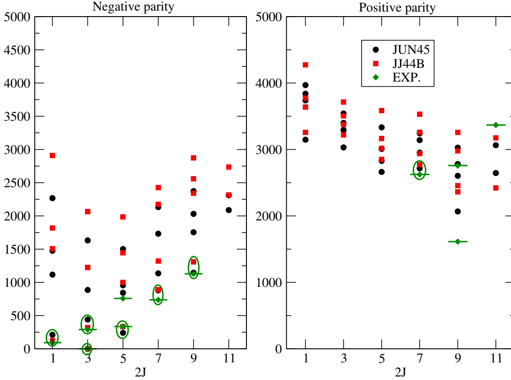
Fig. 10. Comparison between experimental (EXP.) and calculated level schemes for ^{81}\text{As} obtained with two different shell-model interactions (JJ44B and JUN45). Negative parity states are represented on the left hand side and positive parity ones are on the right hand side. Indicated EXP. values are those for which the J^\pi assignment hypotheses are best established. Green ellipses indicate most probable theory-experiment correspondences.
