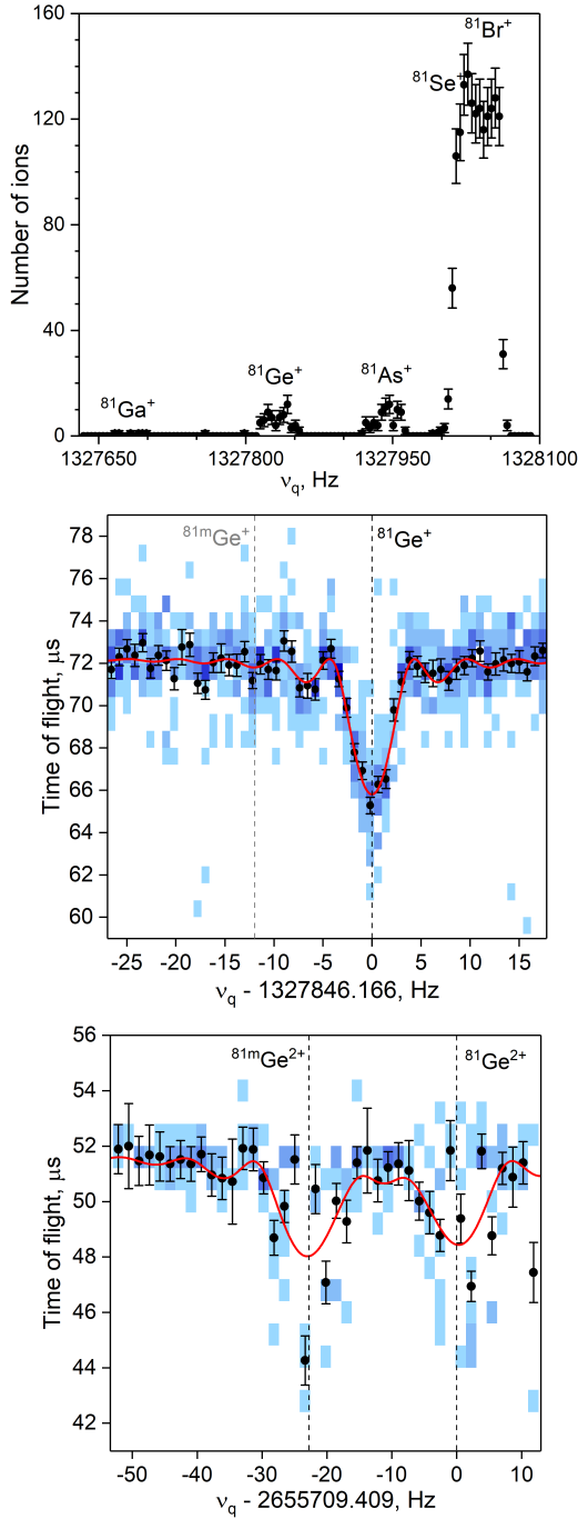
Fig. 1. (top) A quadrupole excitation frequency scan in the first trap of JYFLTRAP showing the isobaric distribution at A = 81 . (middle) A ToF-ICR spectrum for ^{81}\text{Ge}^+ ions using 200 ms quadrupolar excitation in the second trap of JYFLTRAP. (bottom) A ToF-ICR spectrum with 100 ms quadrupolar excitation in the second trap for ^{81}\text{Ge}^{2+} ions after the in-trap \beta -decay of ^{81}\text{Ga} . The ground- and isomeric-state frequencies are indicated with dashed lines in (middle) and (bottom). Blue shaded points are the actual data points, black points represent their mean value with a 1\sigma error bar.
