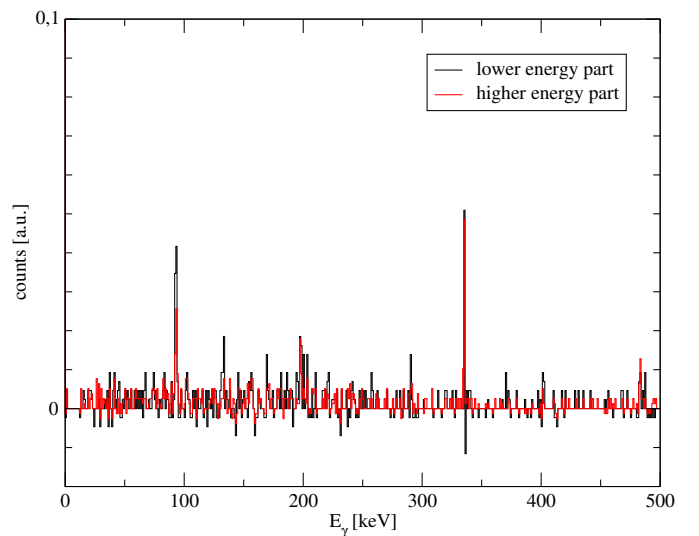
Fig. 7. Normalised \gamma spectra obtained by gating on the lower (black) or higher (red) energy part of the 666-keV peak in the \beta -gated \gamma - \gamma coincidence matrix with identical background subtraction. I(93 \text{ keV})/I(336 \text{ keV})=2.2(9) for lower energy gate and I(93 \text{ keV})/I(336 \text{ keV})=0.9(2) for higher energy part.
