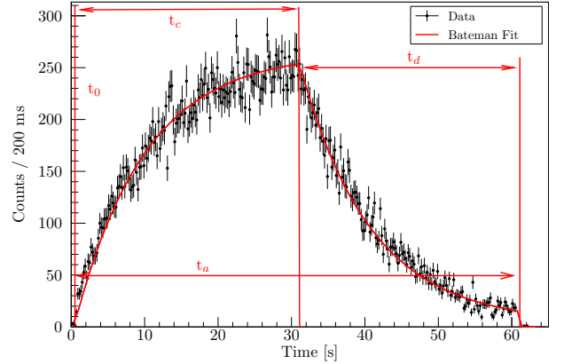
Fig. 2. Time distribution of the background-subtracted \gamma -ray events corresponding to the 335.9(2)-keV transition in ^{81}\text{As} . The Bateman equation fit is shown in red.
