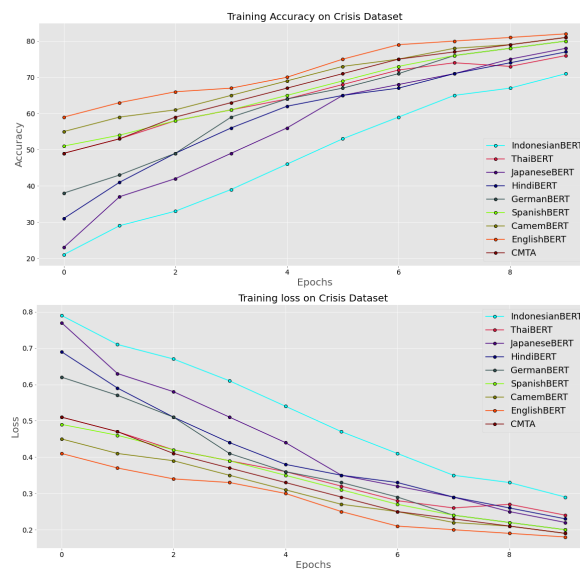
Figure 3: Training Accuracy(Upper) and Training loss(Lower)
