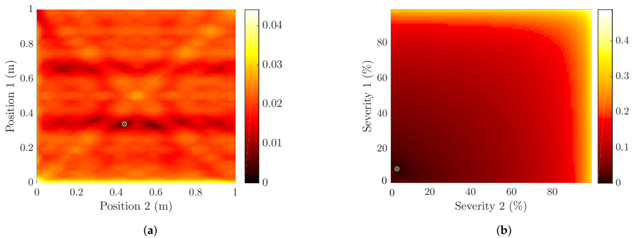
Figure 6. FSC as a function of positions and severity (percentage) where, white circles represent real damaged parameters. Cross symbols and color bars indicate the lowest minimized value. (a) Damage positions are located at 0.34 m and 0.44 m, and (b) the severity of the localized damage is estimated at 9% and 4%, respectively.
