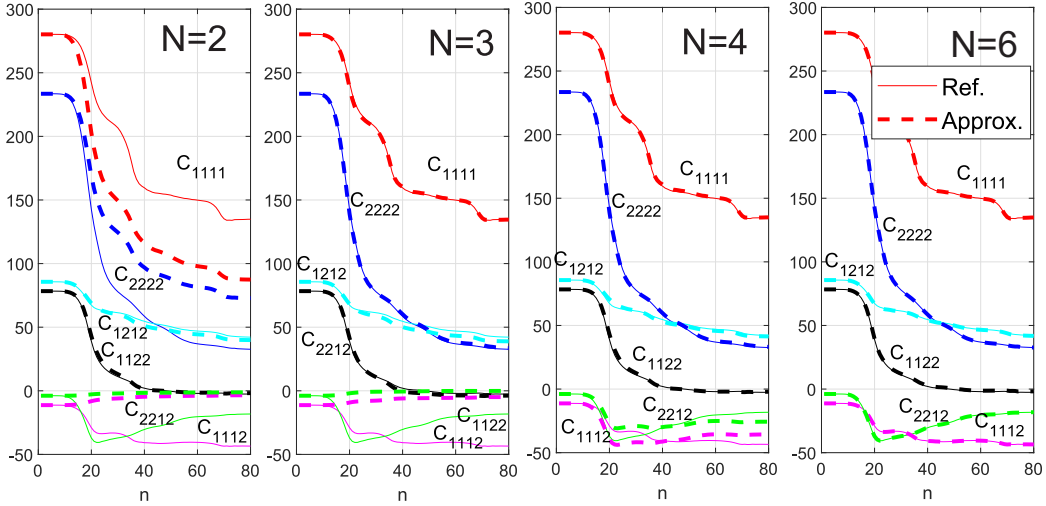
Figure 10. 2D RVE D: comparison between direct numerical simulation (reference) and approximation of the effective elasticity tensor using N internal variables.
