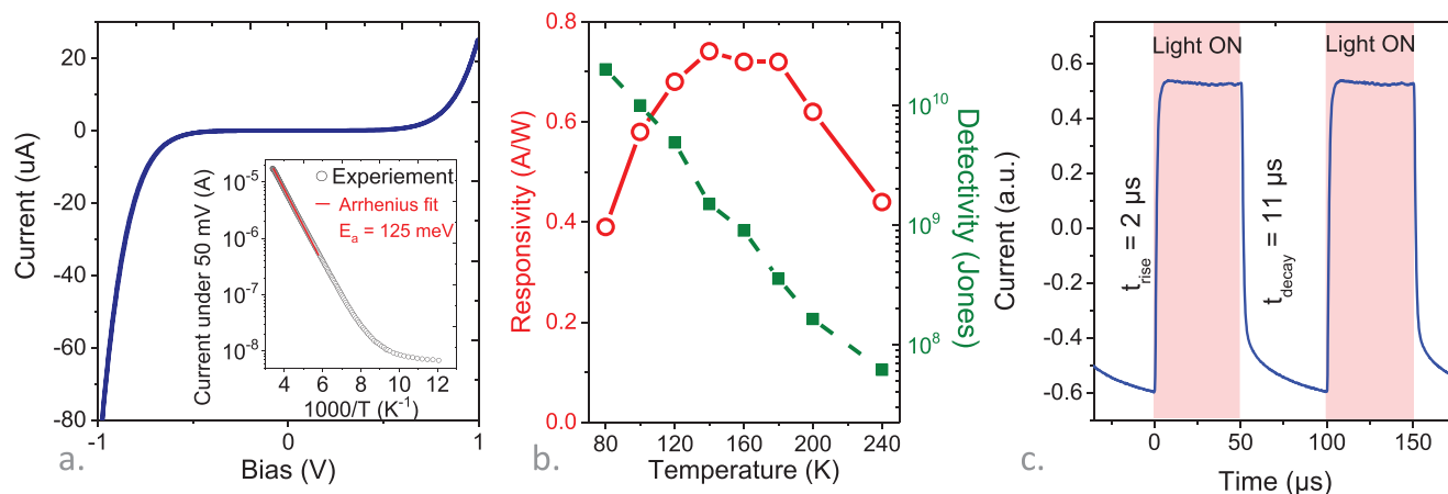
Figure 5. Device performances. a) IV curve of the device at 80 K. The inset is the I-T curve, whose part close to room temperature is fitted with an Arrhenius law, presenting a 125 meV activation energy. b) Responsivity (under broadband blackbody radiation operated at 980^\circ\text{C} ) and detectivity of the device as a function of the device operating temperature when the applied bias is 0.2 V and the light is modulated at 1 kHz. c) Current as a function of time while the device is illuminated with laser pulses ( \lambda = 2.5 \mu\text{m} ).
