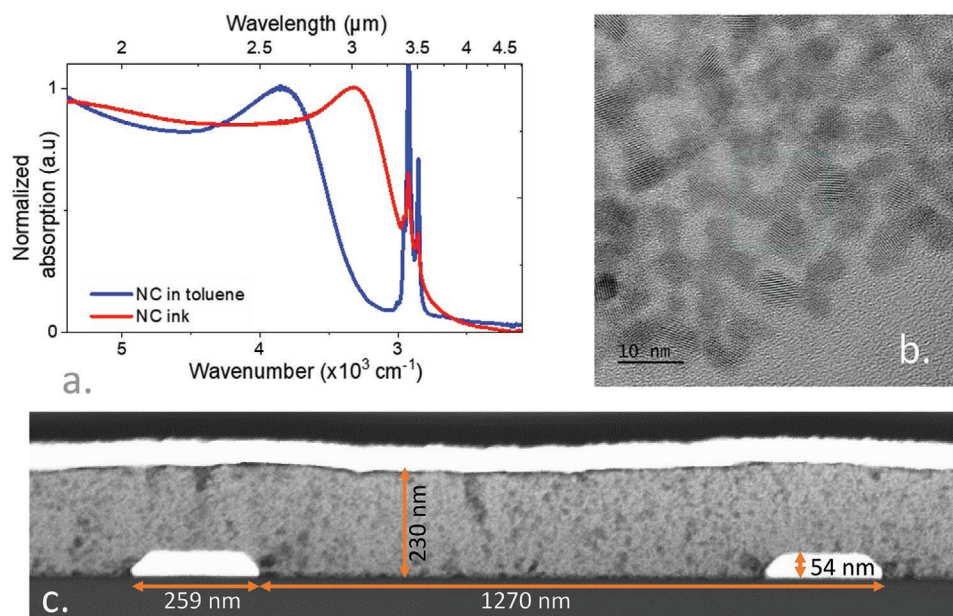
Figure 3. Characterization of the nanocrystal film and device. a) Absorption of HgTe NCs in solution (DDT capped) and under ink form (HgCl 2 -MpOH capped). b) TEM image of the HgTe NC presenting MWIR absorption. c) TEM image of a side view of the device.
