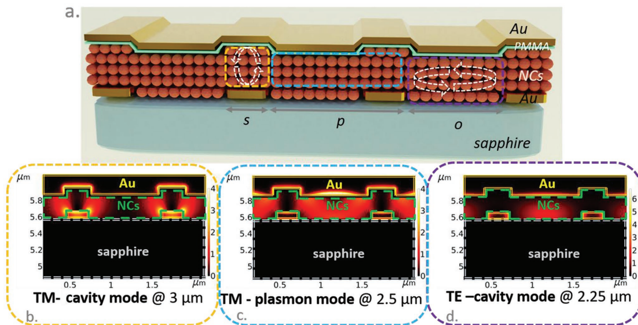
Figure 1. Multi-resonant absorption design. a) Schematic of the multi-resonant MWIR absorbing device. Arrows indicate the regions where cavities are formed due to an impedance mismatch between single and double metal regions. b) Absorption map of the device at 3 \mu\text{m} corresponding to the TM cavity mode resonance wavelength. c) Absorption map of the device at 2.5 \mu\text{m} corresponding to the TM surface plasmon mode wavelength. d) Absorption map of the device at 2.25 \mu\text{m} corresponding to the TE mode resonance wavelength. For parts (b)–(d), the color scale corresponds to the absorption magnitude (in arbitrary units). Electric field maps are provided in Figure S3 (Supporting Information). All the parameters employed for electromagnetic simulations are summarized in paragraph S1.1 (Supporting Information).
