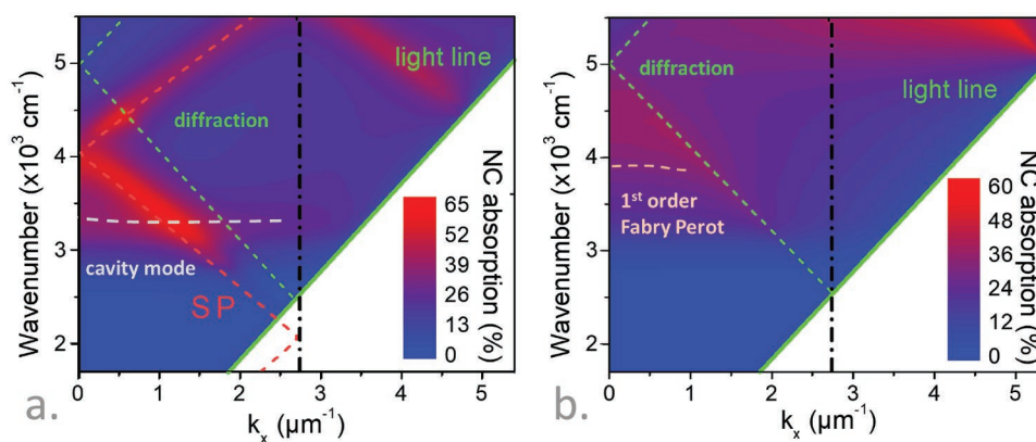
Figure 2. Spectroscopic properties of a multi-resonant structure. a,b) Calculated NC absorption (in color scale) as a function of the photon wavenumber and wavevector in the x direction for TM (resp. TE) polarization. All the parameters employed for electromagnetic simulations are summarized in paragraph S1.1 (Supporting Information). The continuous green line is the light line in the sapphire, while the green dashed lines represent its diffracted orders. The dashed red line represents the calculated SP polariton dispersion, together with its diffracted orders. The vertical black line indicates the edge of the first Brillouin zone, at k_x = \pi/p . The horizontal white dashed lines represent the Fabry–Perot cavity modes.
