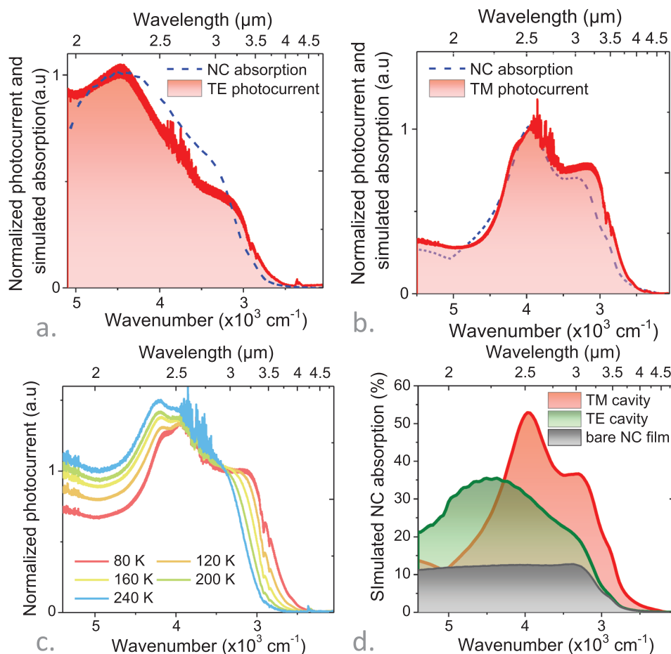
Figure 4. Broadband absorption in the short and mid-wave infrared. a,b) Simulated NC absorption and experimental photocurrent spectra under TE (resp. TM) polarization, at 80 K. c) Experimental unpolarized photocurrent spectra at various temperatures. d) Simulated absorption spectra for the bare NC film and the same film introduced in our multi-resonant geometry.
