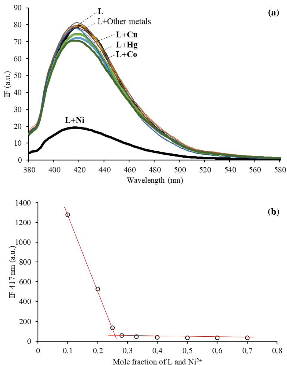
Figure 1: (a) Emission fluorescence spectra ( \lambda_{\text{exc}} = 340\text{nm} ) of L (10 \mu\text{M} ) in phosphate buffer (pH=7) and L with addition of various metal ions \text{M} ( \text{M}:\text{L}_3 ratio); (b) Job's plot analysis of L (10 \mu\text{M} ) regarding \text{Ni}^{2+} ion (10 \mu\text{M} ).
