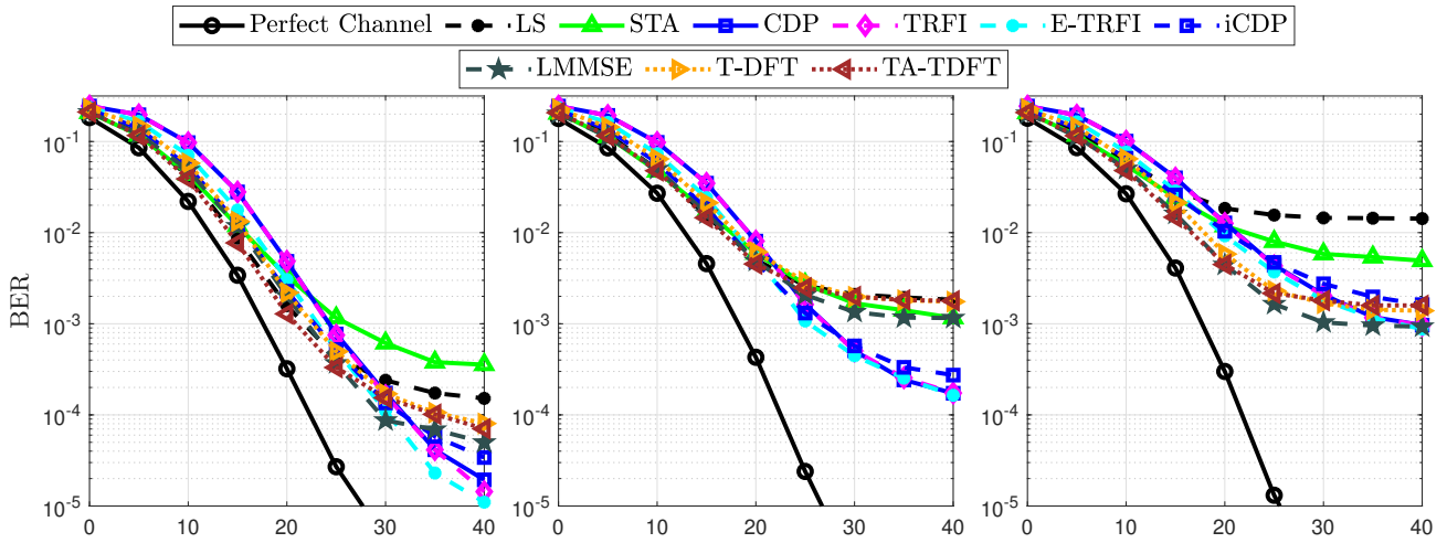
(a) BER performance with I = 10 .
