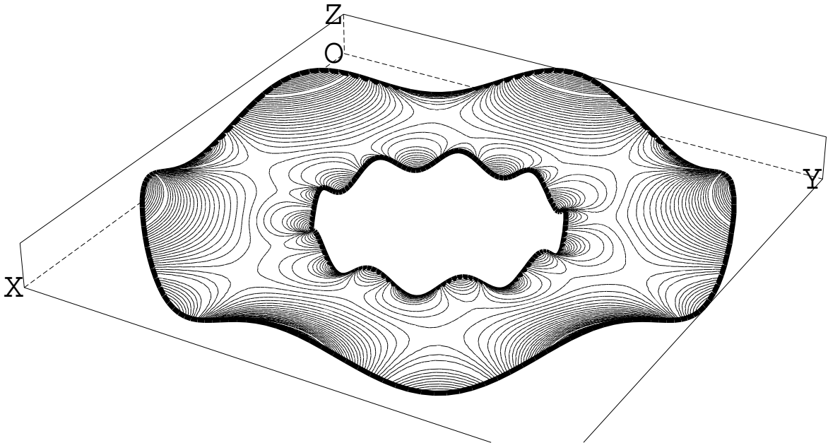
Figure 23. Minimal usual variational surface.
