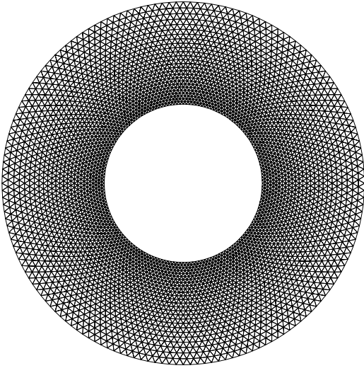
Figure 22. Uniform mesh.
