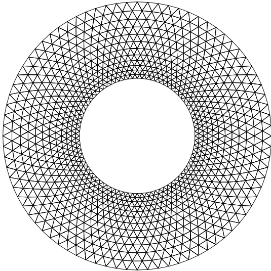
Figure 1. Equilateral mesh.
