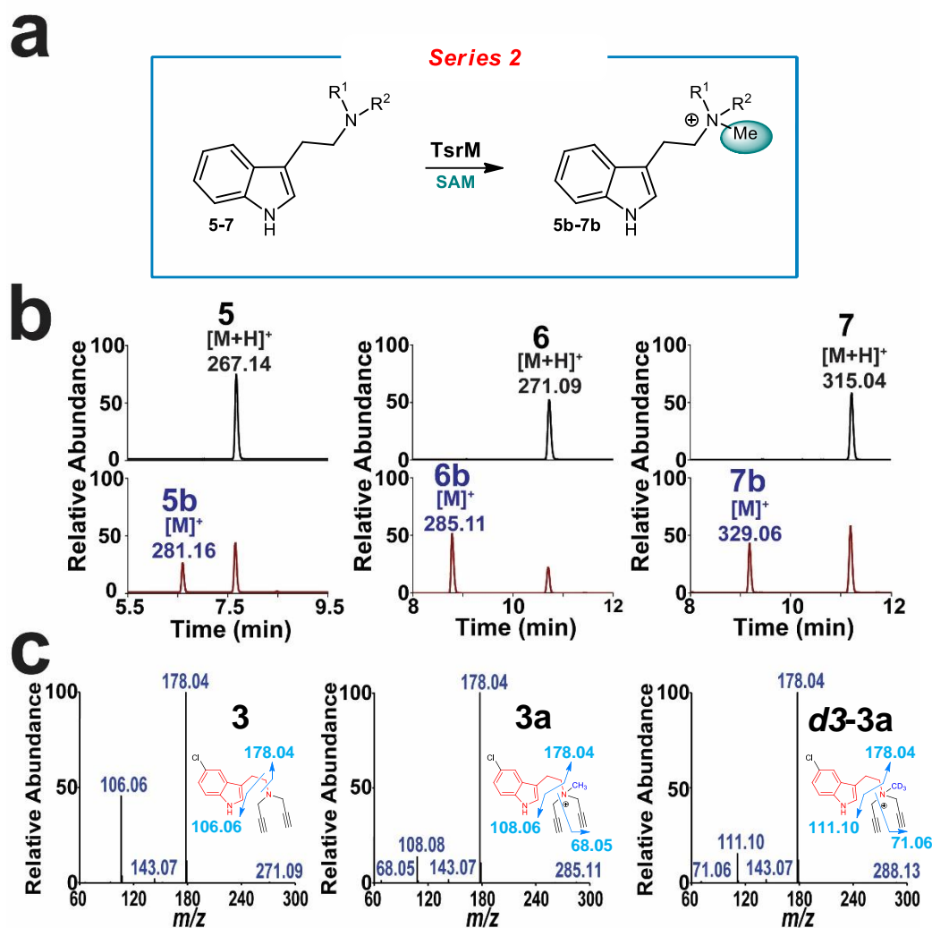
Figure 8. Activity of TsrM on tryptamine di-propargyl derivatives. (a) Reaction catalyzed by TsrM on 5-7. (b) LC-MS analysis of the reactions of TsrM with 5 ( m/z=267.14 ), 6 ( m/z=271.09 ) and 7 ( m/z=315.04 ). Methylated products 5b, 6b & 7b were characterized by a mass shift of \Delta m=14 Da. (c) LC-MS/MS analysis of 6 (left panel) and the reaction product 6b obtained in the presence of SAM (middle panel) or d3-SAM (right panel).
