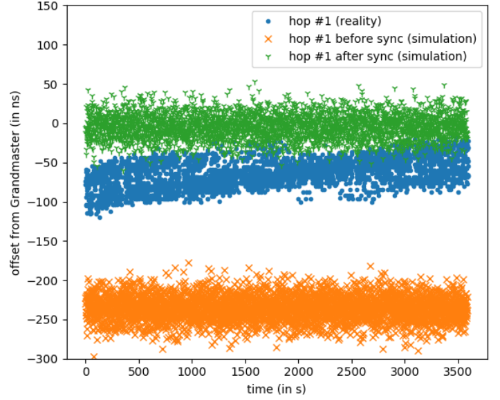
Fig. 11: Offset between the Grandmaster clock and the switch clock at hop #1 in reality and the simulator. The simulator is configured with the granularity, mean link delay and the standard deviation estimated in the previous experiments. For the clock drift, we use the drift measured before each experiment.
