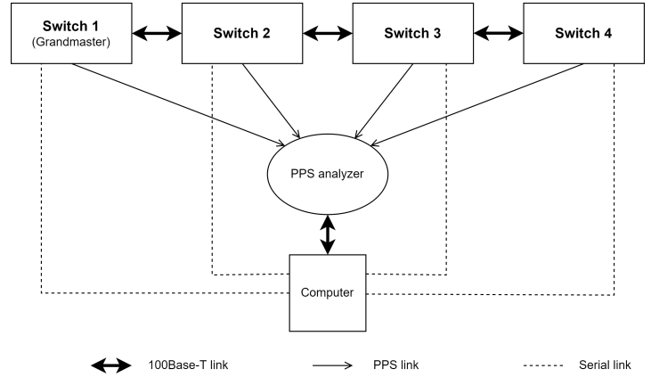
Fig. 3: Experimental measurement topology.
