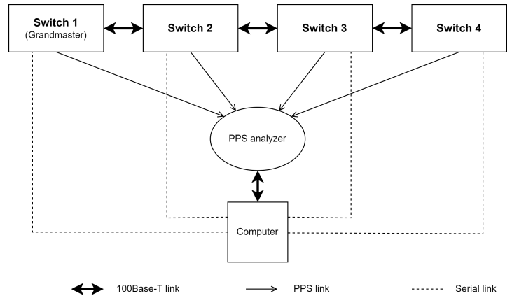
Fig. 3: Experimental measurement topology.
