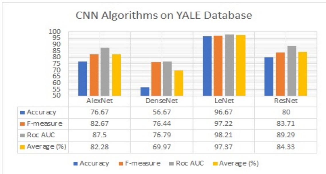
Figure 16: Performance of some CNN algorithms on YALE database.
