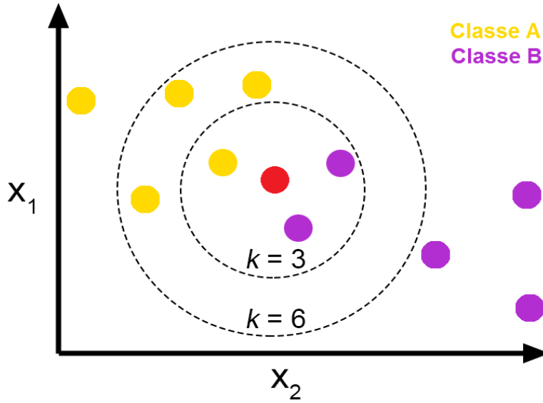
Figure 3: K-Nearest Neighbours Algorithm.
