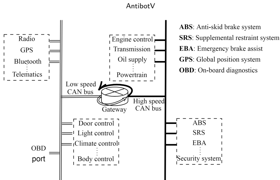
Figure 3: In-vehicle network
