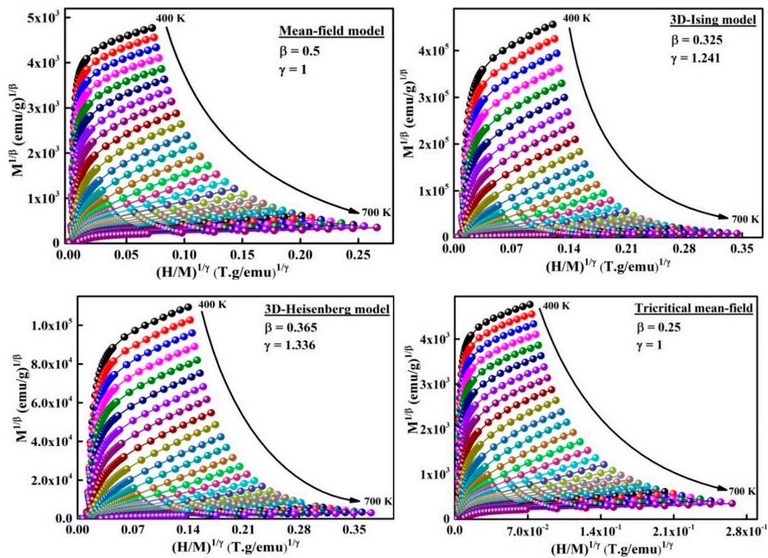
Figure 7. Adapted Arrott plots M^{1/\beta} versus (H/M)^{1/\gamma} from M(H) isotherms.
