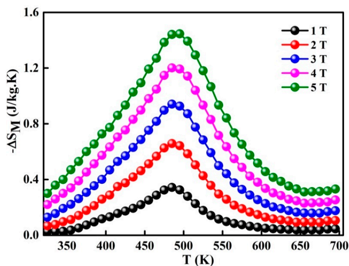
Figure 6. Temperature dependence of change in magnetic entropy for different magnetic fields.
