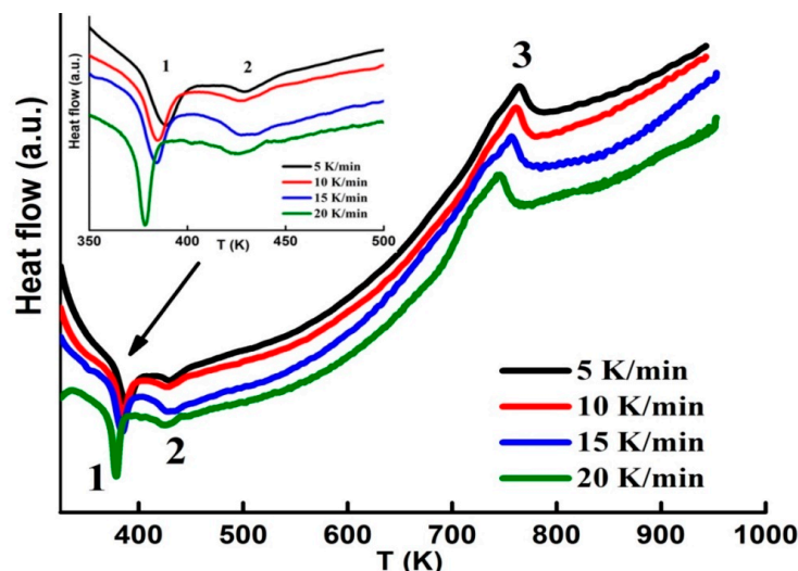
Figure 2. DSC scans measured with several heating rates (the inset shows the first peak). Peaks 1 and 2 correspond to two FM-PM transitions, and peak 3 to the crystallization process.
