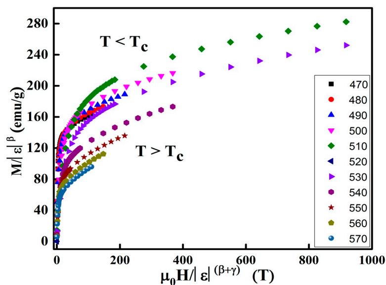
Figure 12. Scaling plots in the vicinity of T_C .
