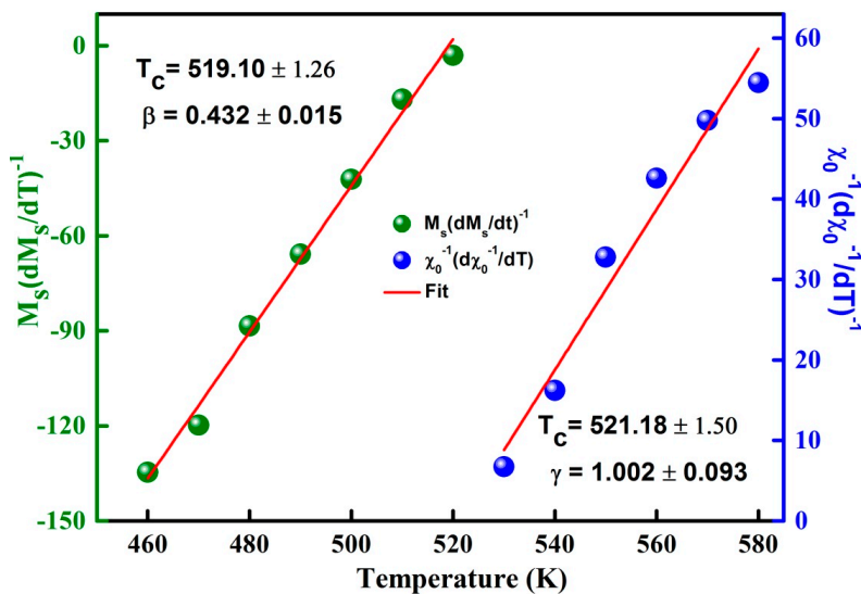
Figure 10. K-F plots of M_S(T)(dM_S(T)/dT)^{-1} and \chi_0^{-1}(T)(d\chi_0^{-1}(T)/dT)^{-1} versus T .
