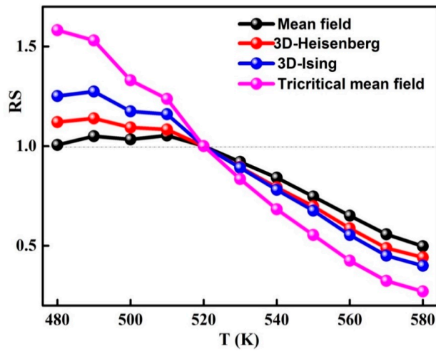
Figure 8. Temperature reliance of the relative slope ( RS = S(T)/S(T_c) ) for different models.
