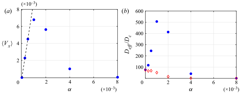
Figure 4. (a) The x -component of the Lagrangian velocity \langle V_x \rangle and (b) non-dimensional effective diffusion D_{eff}^x/D_c , for Pe_s = 314 , Pe_c = 15\,708 as a function of \alpha . ( \bullet , blue) x -direction; ( \diamond , red) y -direction.
